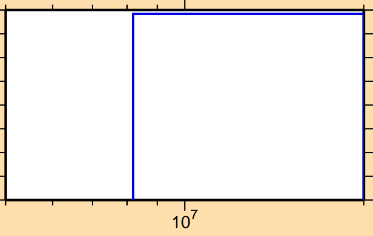
\sigma vs. E for ^{107}\text{Cd}(n,\text{pd})
