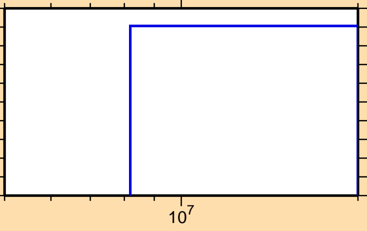
\sigma vs. E for ^{107}\text{Cd}(n,\text{He}3)
