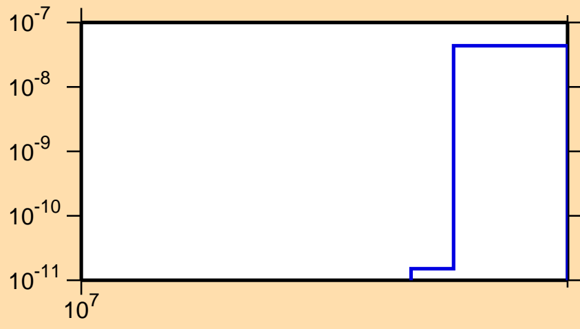
\sigma vs. E for ^{108}\text{Cd}(n,2n\alpha)
