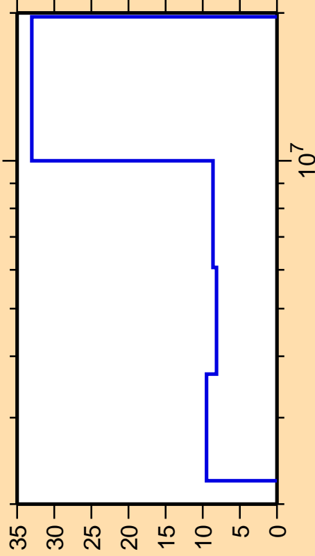
\Delta\sigma/\sigma vs. E for ^{108}\text{Cd}(n,n\text{cont.})
