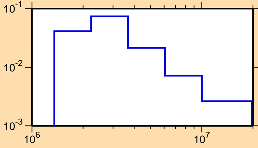
\sigma vs. E for ^{108}\text{Cd}(n,n_4)
