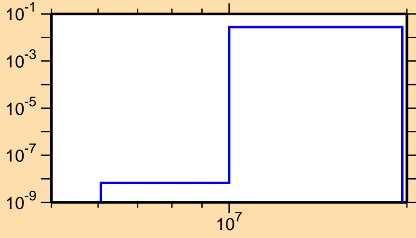
\sigma vs. E for ^{108}\text{Cd}(n,np)
