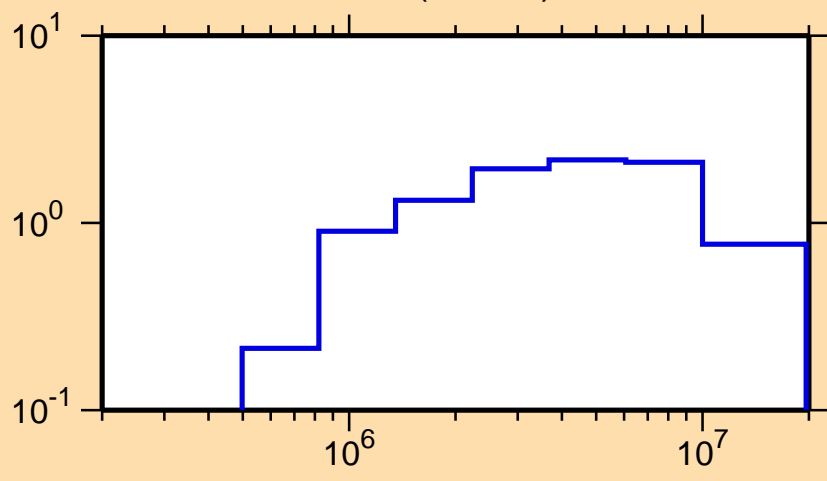
\sigma vs. E for ^{108}\text{Cd}(n,\text{inel.})
