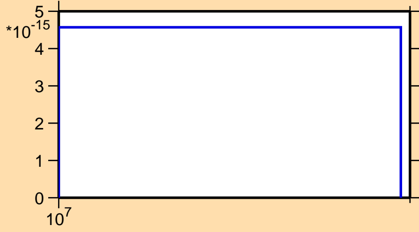
\sigma vs. E for ^{108}\text{Cd}(n,nt)
