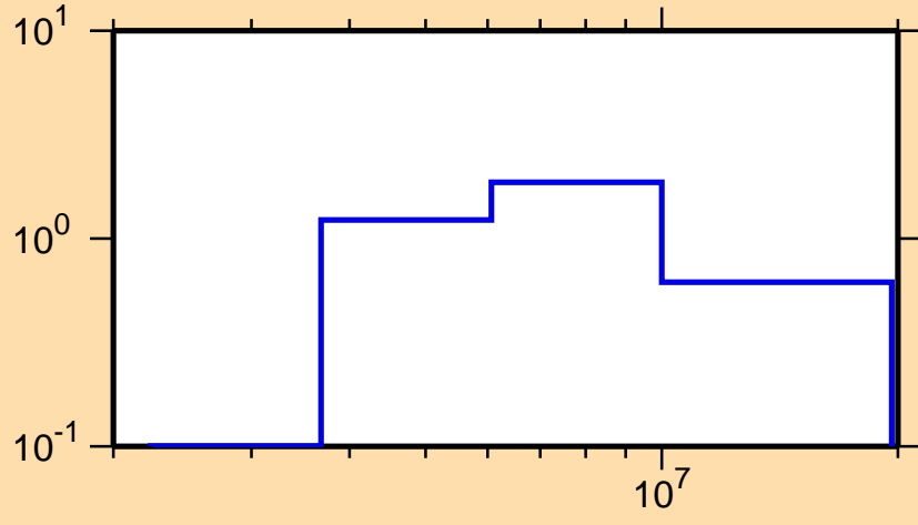
\sigma vs. E for ^{108}\text{Cd}(n,n\text{cont.})
