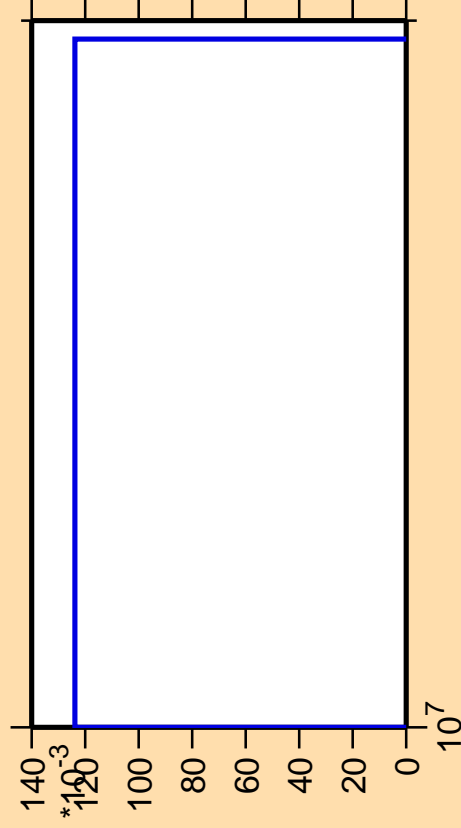
\Delta\sigma/\sigma vs. E for ^{108}\text{Cd}(\text{mt117})
