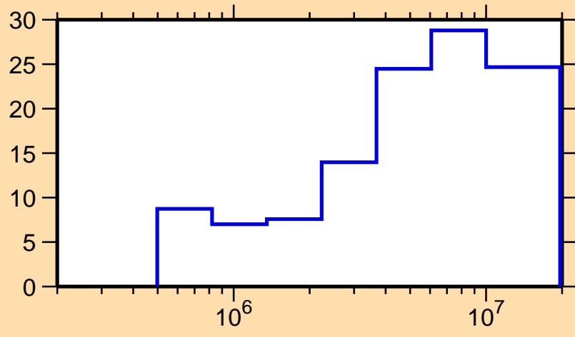
\Delta\sigma/\sigma vs. E for ^{108}\text{Cd}(n,n_1)
