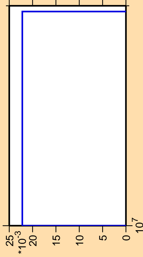
\Delta\sigma/\sigma vs. E for ^{108}\text{Cd}(n,nt)
