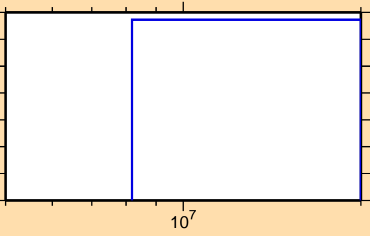
\sigma vs. E for ^{108}\text{Cd}(n,\text{He}3)
