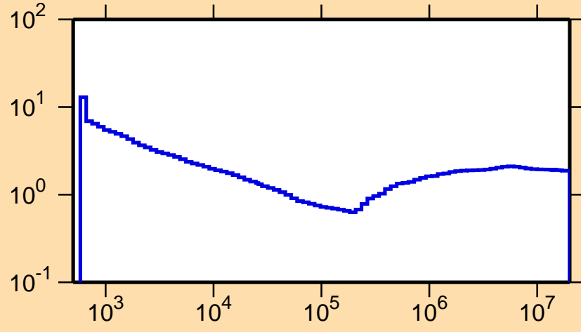
\sigma vs. E for ^{109}\text{Cd}(n,\text{nonel.})
