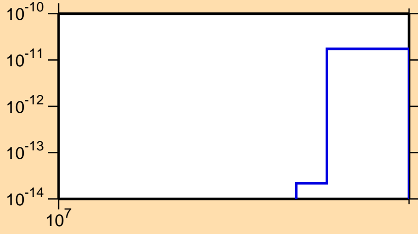
\sigma vs. E for ^{109}\text{Cd}(n,nt)
