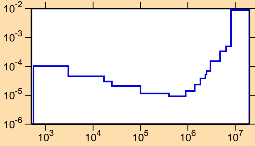
\sigma vs. E for ^{109}\text{Cd}(n,\alpha)
