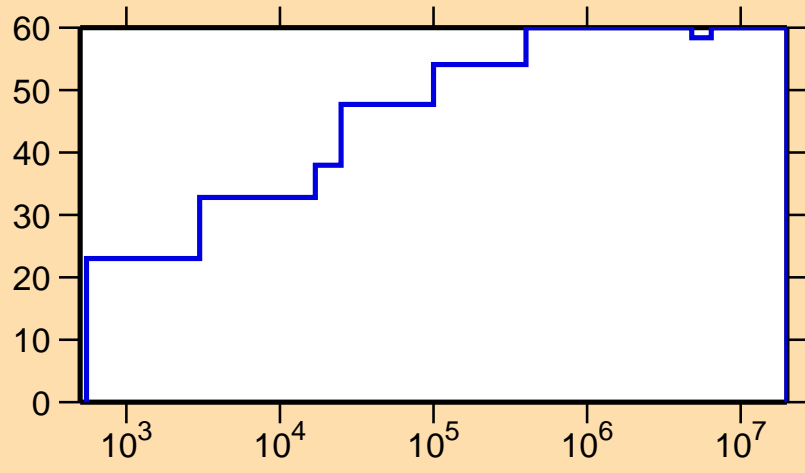
\Delta\sigma/\sigma vs. E for ^{109}\text{Cd}(n,\gamma)
