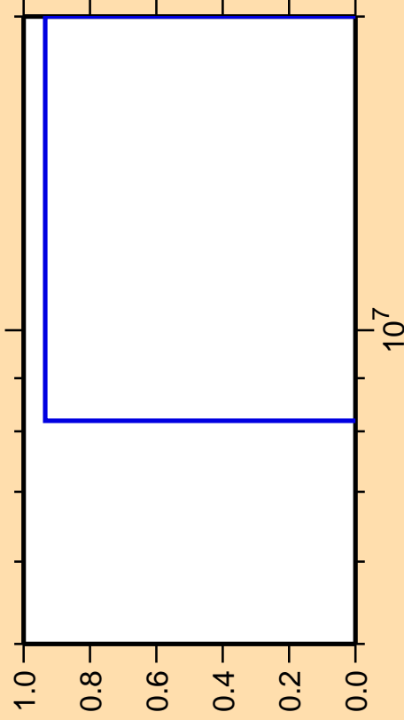
\Delta\sigma/\sigma vs. E for ^{109}\text{Cd}(n,nt)
