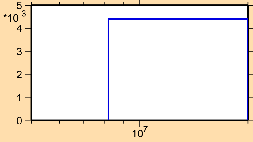
\sigma vs. E for ^{109}\text{Cd}(n,np)
