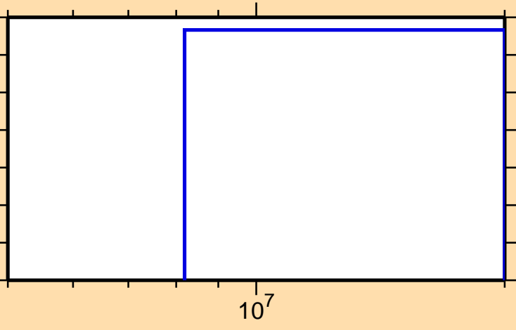
\sigma vs. E for ^{109}\text{Cd}(n,\text{He3})
