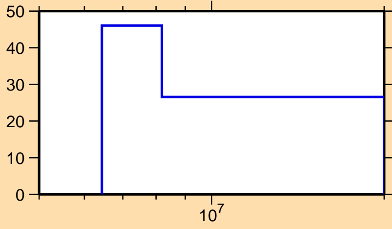
\Delta\sigma/\sigma vs. E for ^{109}\text{Cd}(n,2n)
