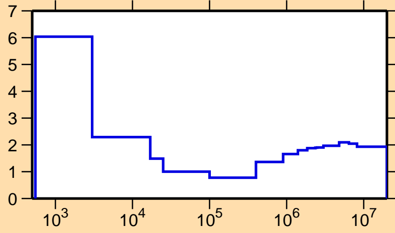
\sigma vs. E for ^{109}\text{Cd}(n,\text{nonel.})
