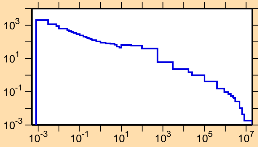
\sigma vs. E for ^{109}\text{Cd}(n,\gamma)
