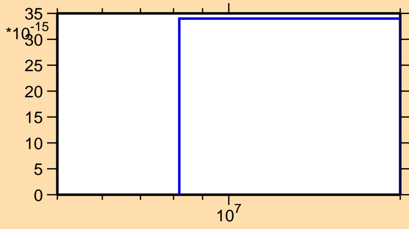
\sigma vs. E for ^{109}\text{Cd}(n,\text{pt})
