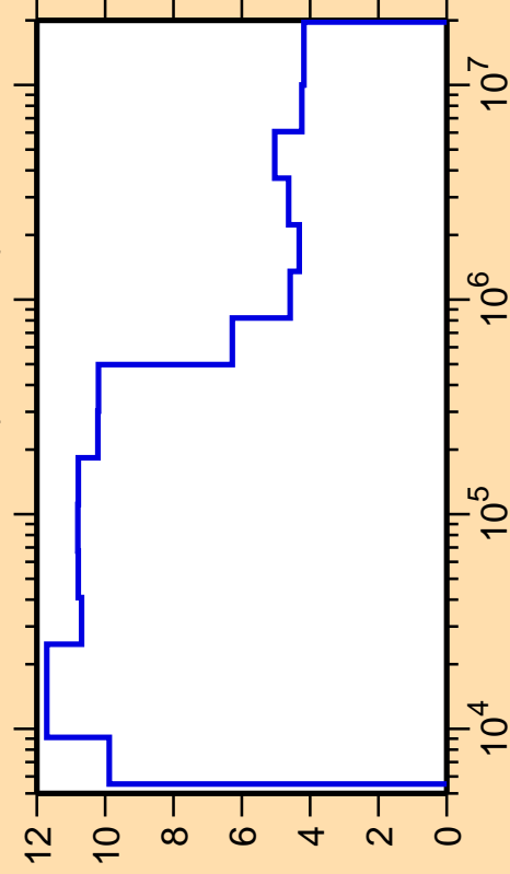
\Delta\sigma/\sigma vs. E for ^{110}\text{Cd}(n,\text{nonel.})
