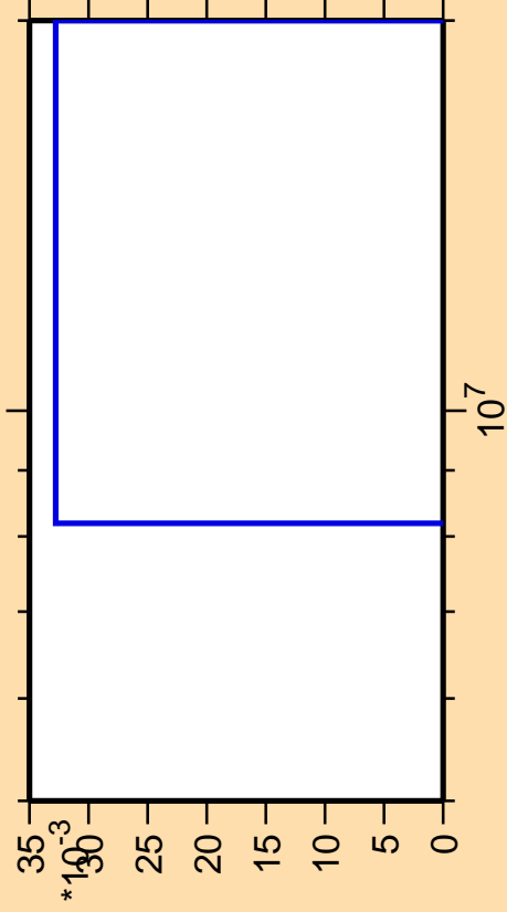
\Delta\sigma/\sigma vs. E for ^{110}\text{Cd}(n,pd)
