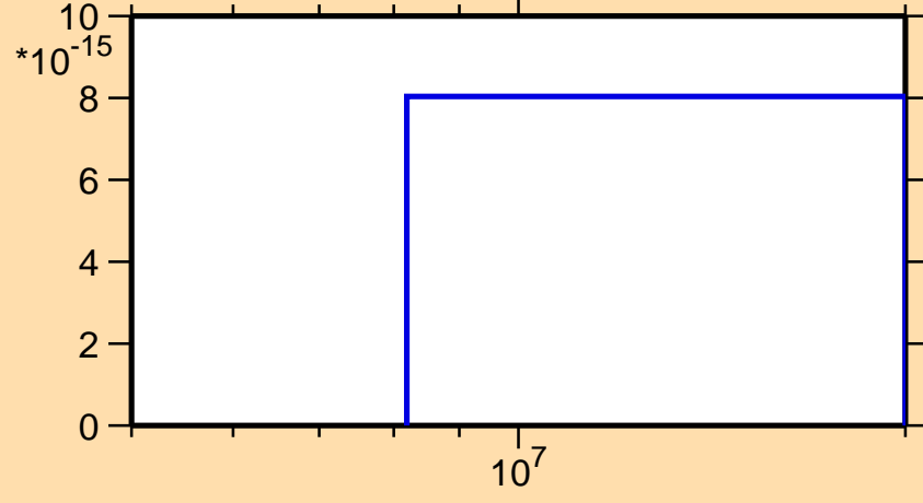
\sigma vs. E for ^{110}\text{Cd}(n,pd)
