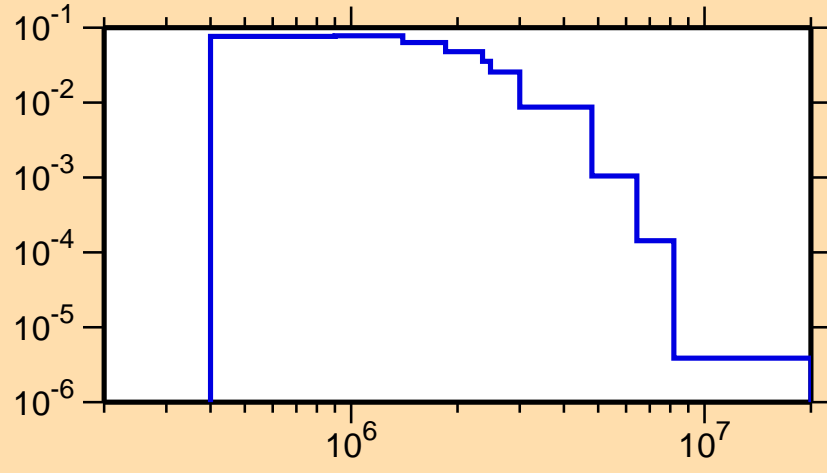
\sigma vs. E for ^{111}\text{Cd}(n,n_4)
