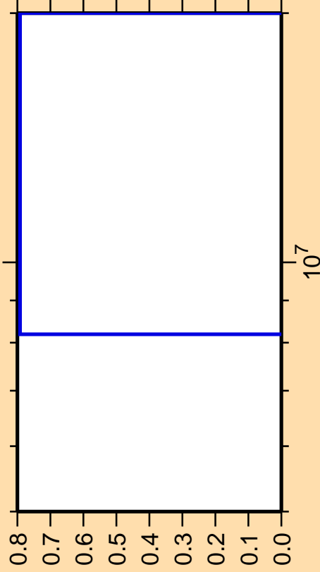
\Delta\sigma/\sigma vs. E for ^{111}\text{Cd}(n,nt)
