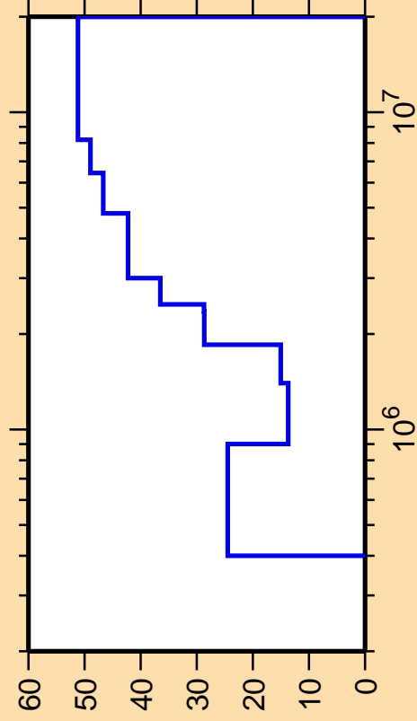
\Delta\sigma/\sigma vs. E for ^{111}\text{Cd}(n,n_4)
