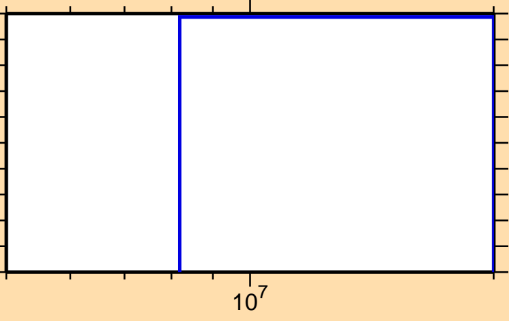
\sigma vs. E for ^{111}\text{Cd}(n,\text{nd})
