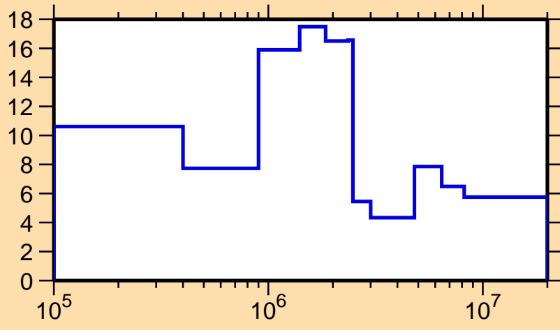
Δσ/σ vs. E for ^{111}\text{Cd}(n,\text{el.})
