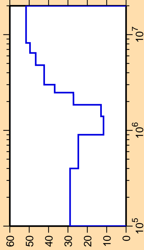
\Delta\sigma/\sigma vs. E for ^{111}\text{Cd}(n,n_2)
