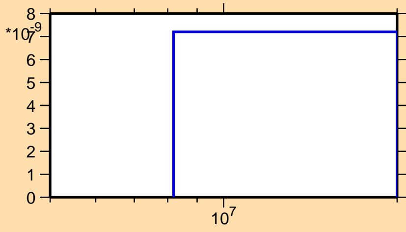
\sigma vs. E for ^{111}\text{Cd}(n,2n\alpha)
