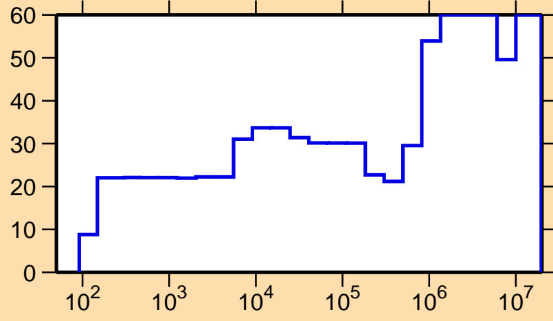
\Delta\sigma/\sigma vs. E for ^{111}\text{Cd}(n,\gamma)
