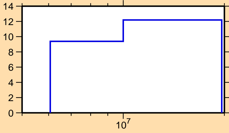
\Delta\sigma/\sigma vs. E for ^{111}\text{Cd}(n,\text{el.})
