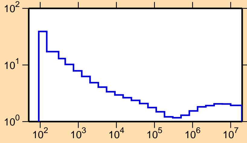
\sigma vs. E for ^{111}\text{Cd}(n,\text{nonel.})
