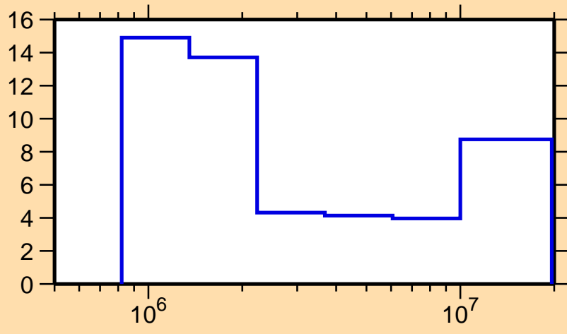
\Delta\sigma/\sigma vs. E for ^{111}\text{Cd}(n,\text{tot.})
