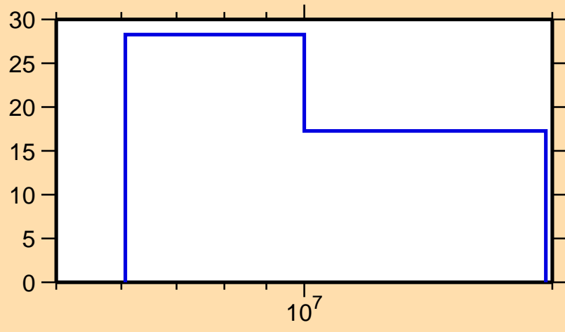
\Delta\sigma/\sigma vs. E for ^{111}\text{Cd}(n,2n)
