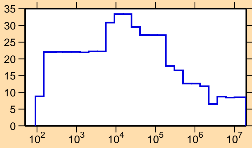
\Delta\sigma/\sigma vs. E for ^{111}\text{Cd}(n,\text{nonel.})
