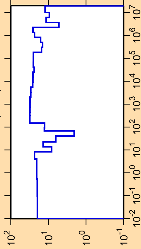
\Delta\sigma/\sigma vs. E for ^{111}\text{Cd}(n,\text{el.})
