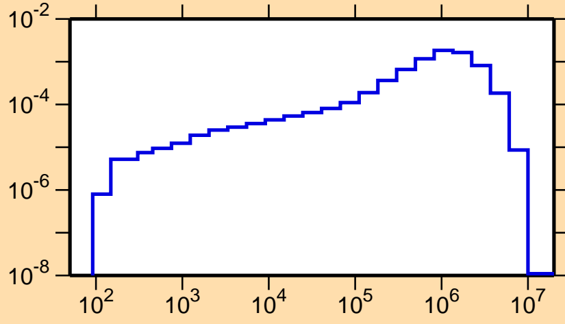
\sigma vs. E for ^{111}\text{Cd}(n,n_1)
