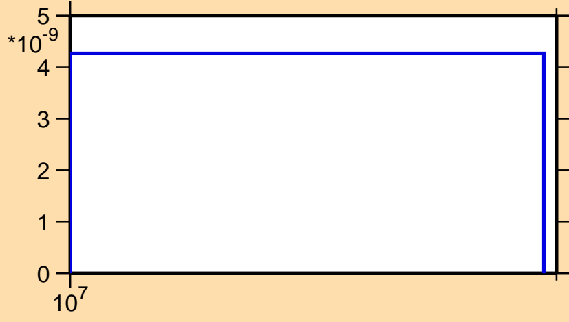
\sigma vs. E for ^{111}\text{Cd}(n,2np)
