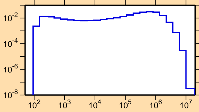
\sigma vs. E for ^{111}\text{Cd}(n,n_2)
