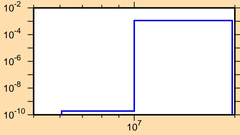
\sigma vs. E for ^{111}\text{Cd}(n,d)
