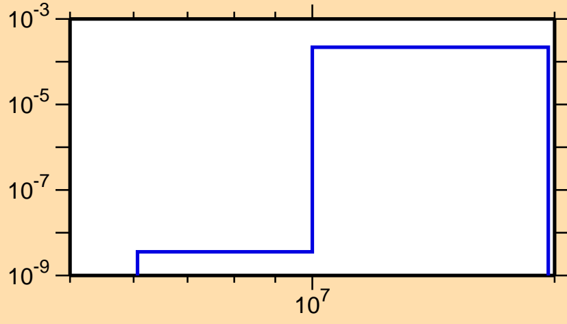
\sigma vs. E for ^{111}\text{Cd}(n,n\alpha)
