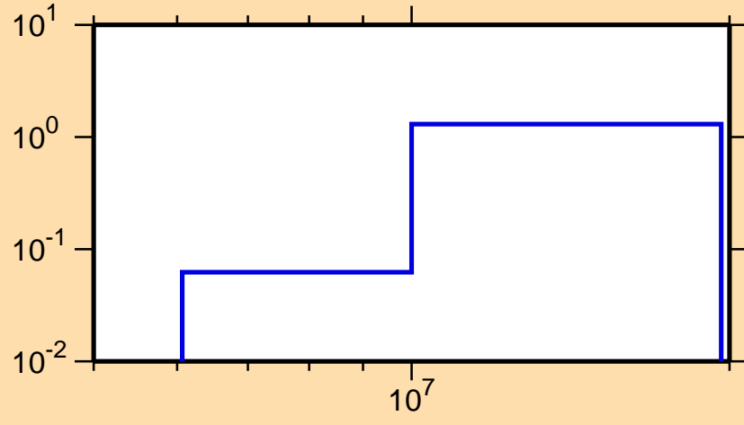
\sigma vs. E for ^{111}\text{Cd}(n,2n)
