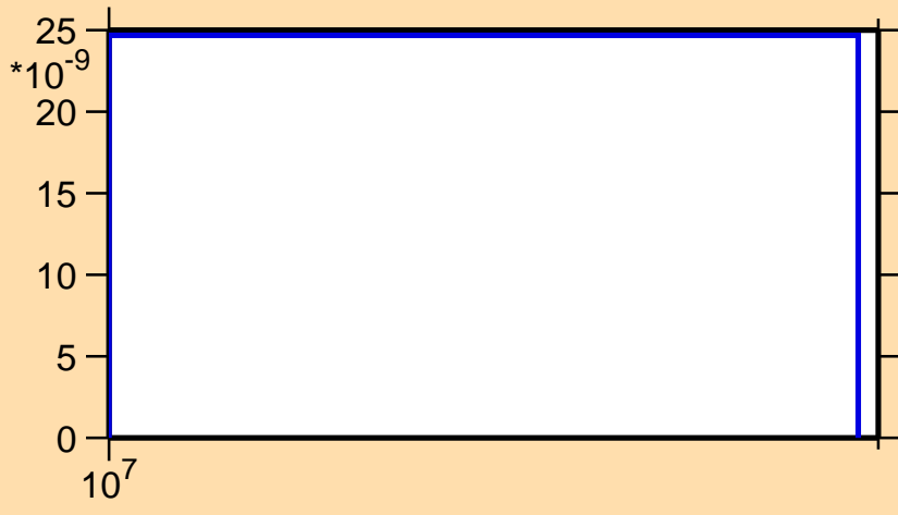
\sigma vs. E for ^{111}\text{Cd}(n,\text{nd})
