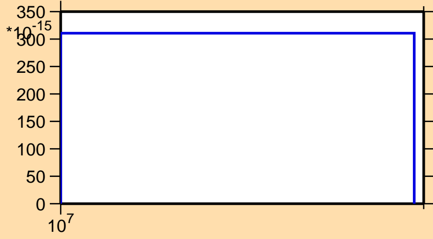
\sigma vs. E for ^{111}\text{Cd}(n,nt)
