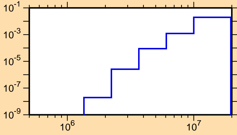
\sigma vs. E for ^{111}\text{Cd}(n,p)
