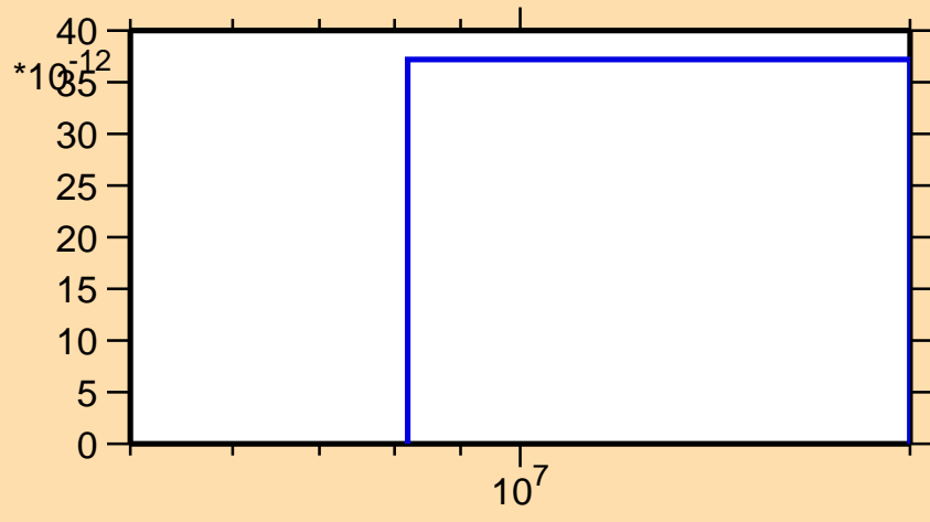
\sigma vs. E for ^{111}\text{Cd}(n,p\alpha)
