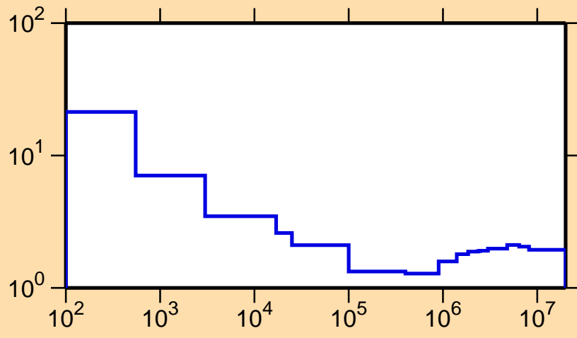
\sigma vs. E for ^{111}\text{Cd}(n,\text{nonel.})
