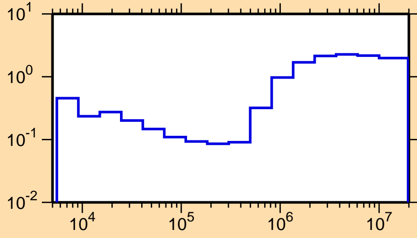
\sigma vs. E for ^{112}\text{Cd}(n,\text{nonel.})
