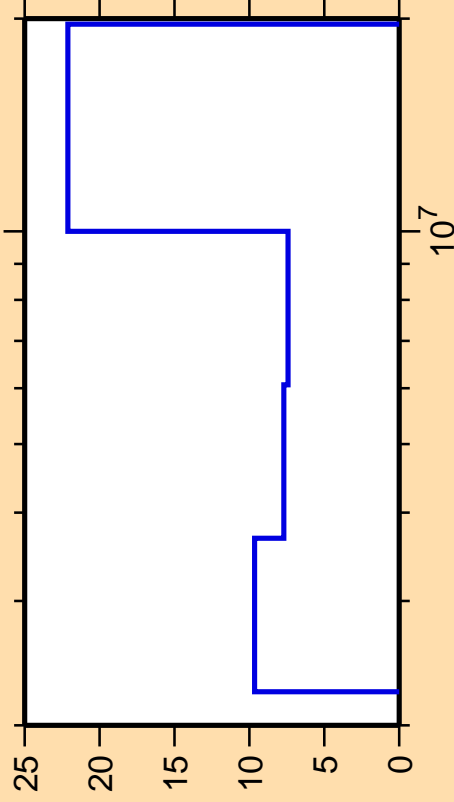
\Delta\sigma/\sigma vs. E for ^{112}\text{Cd}(n,n\text{cont.})
