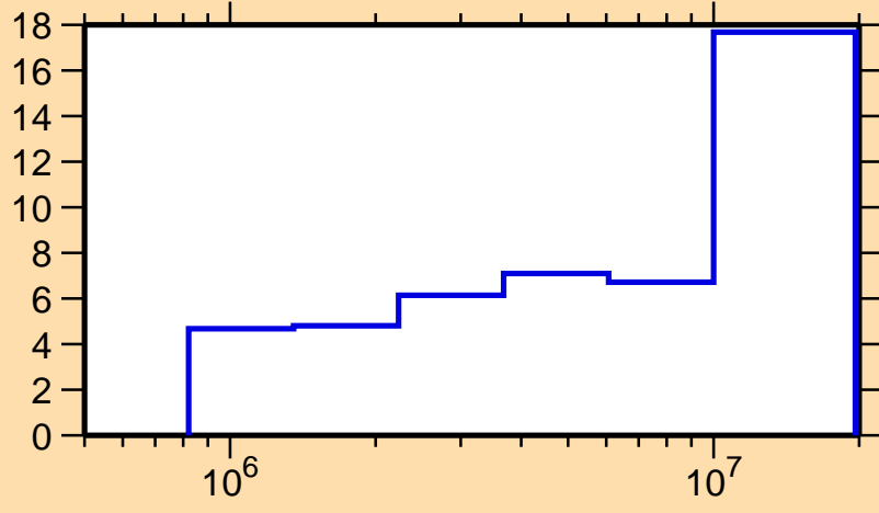
\Delta\sigma/\sigma vs. E for ^{112}\text{Cd}(n,\text{inel.})
