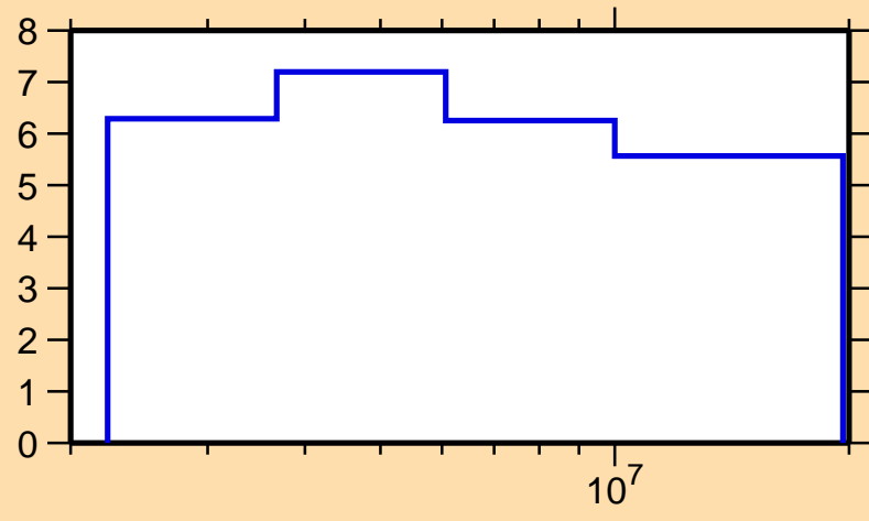
\Delta\sigma/\sigma vs. E for ^{112}\text{Cd}(n,n\text{onel.})
