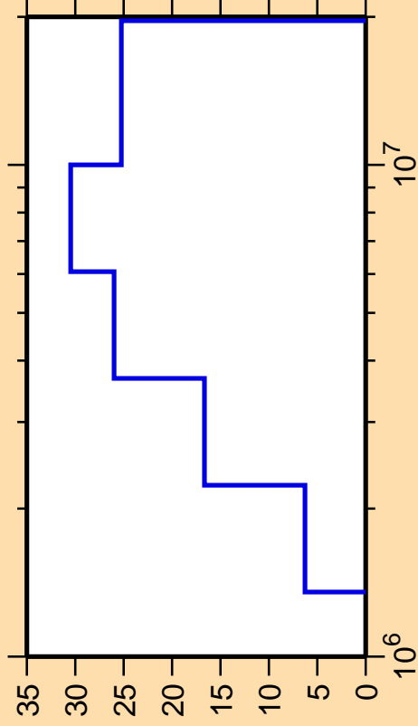
\Delta\sigma/\sigma vs. E for ^{112}\text{Cd}(n,n_4)
