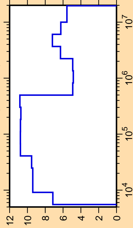
\Delta\sigma/\sigma vs. E for ^{112}\text{Cd}(n,\text{nonel.})
