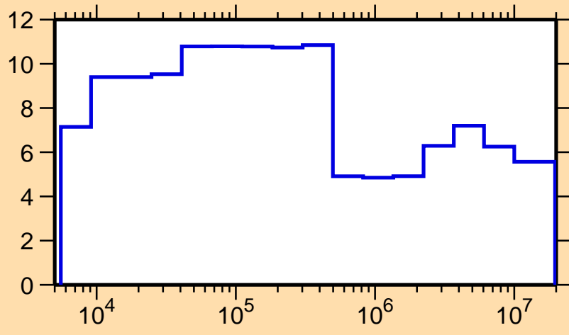
\Delta\sigma/\sigma vs. E for ^{112}\text{Cd}(n,\text{nonel.})
