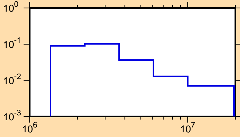
\sigma vs. E for ^{112}\text{Cd}(n,n_4)
