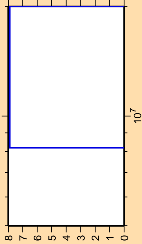
\Delta\sigma/\sigma vs. E for ^{112}\text{Cd}(n,2n\alpha)
