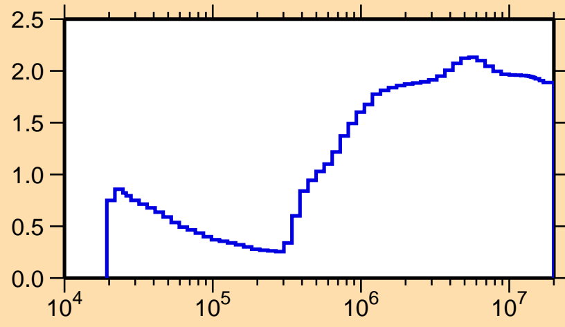
\sigma vs. E for ^{113}\text{Cd}(n,\text{nonel.})
