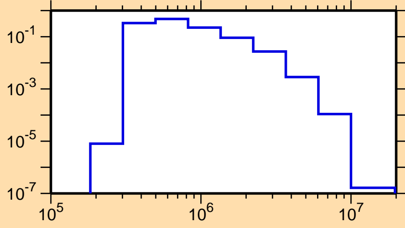
\sigma vs. E for ^{113}\text{Cd}(n,n_2)
