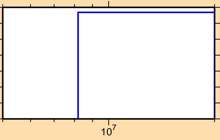
\sigma vs. E for ^{113}\text{Cd}(n,\text{nd})
