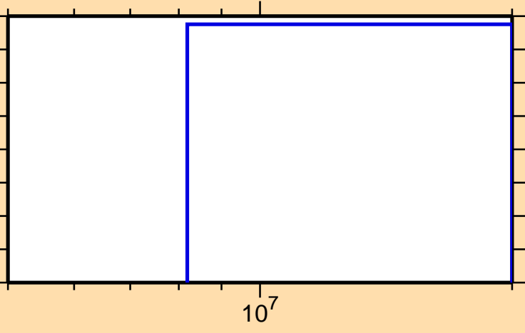
\sigma vs. E for ^{113}\text{Cd}(n,np)
