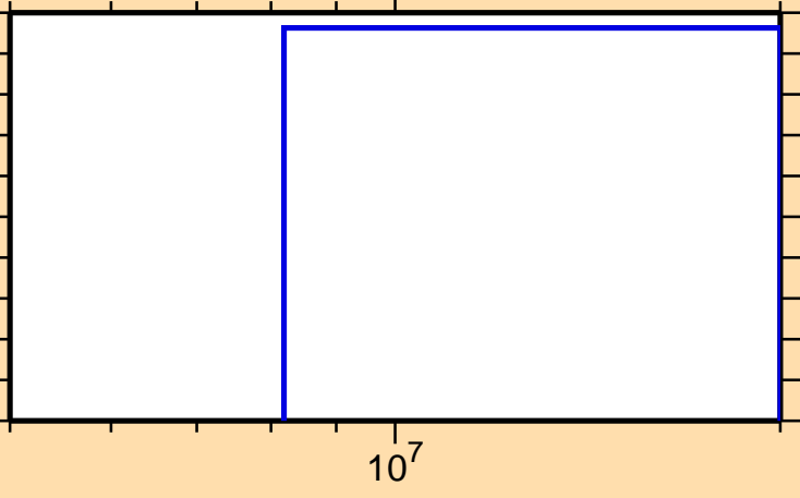
\sigma vs. E for ^{113}\text{Cd}(n,t)
