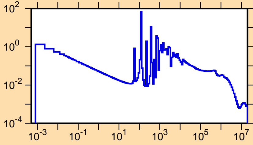
\sigma vs. E for ^{114}\text{Cd}(n,\gamma)
