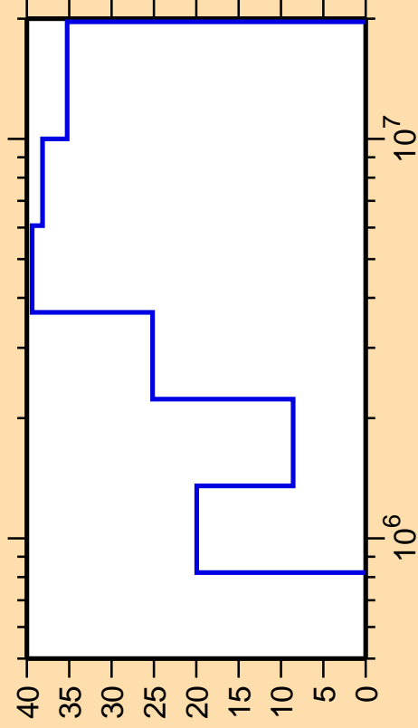
\Delta\sigma/\sigma vs. E for ^{114}\text{Cd}(n,n_4)
