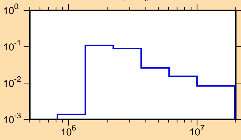
\sigma vs. E for ^{114}\text{Cd}(n,n_4)
