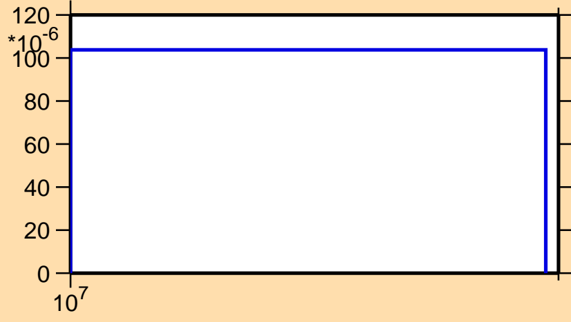
\sigma vs. E for ^{114}\text{Cd}(n,np)
