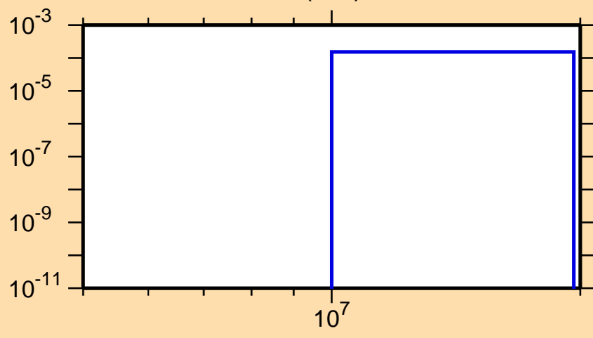
\sigma vs. E for ^{114}\text{Cd}(n,d)
