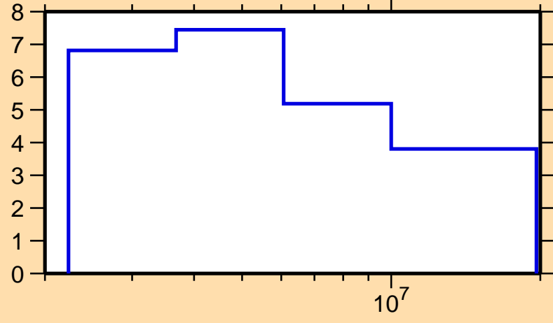
\Delta\sigma/\sigma vs. E for ^{114}\text{Cd}(n,n\text{onel.})
