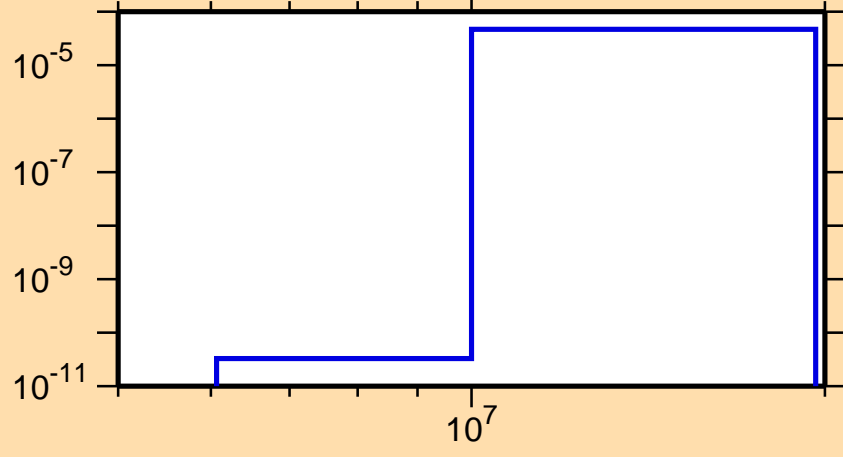
\sigma vs. E for ^{114}\text{Cd}(n,n\alpha)
