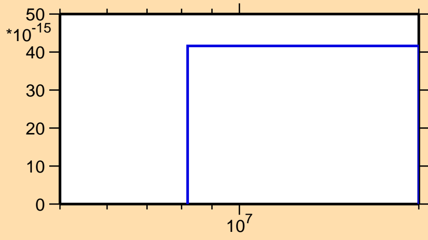
\sigma vs. E for ^{114}\text{Cd}(n,\text{He}3)
