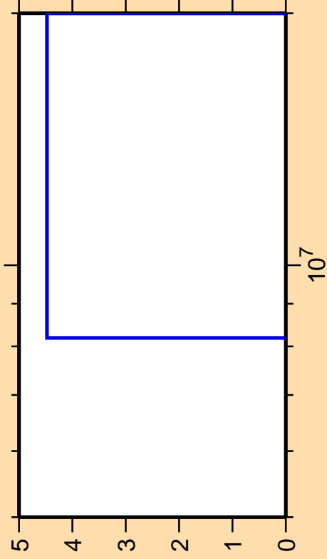
\Delta\sigma/\sigma vs. E for ^{114}\text{Cd}(n,2n\alpha)
