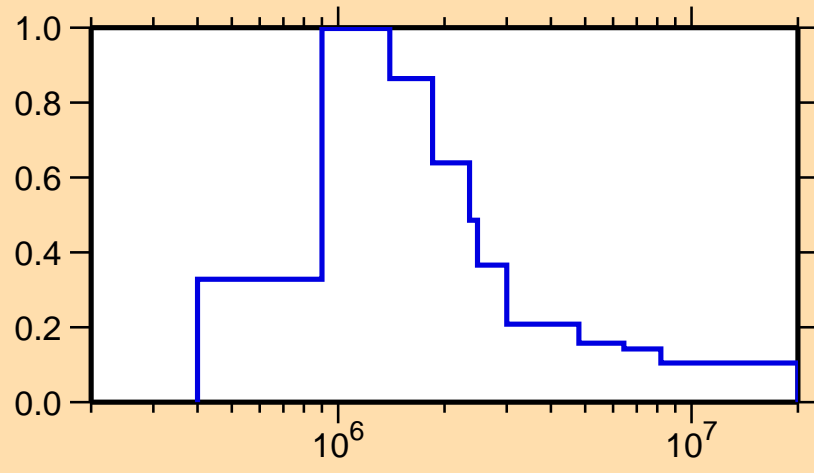
\sigma vs. E for ^{114}\text{Cd}(n,n_1)
