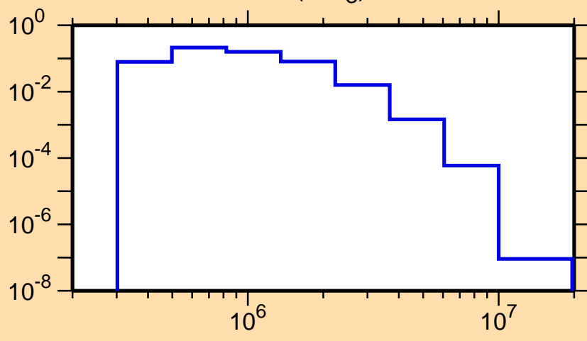
\sigma vs. E for ^{115}\text{Cd}(n,n_3)
