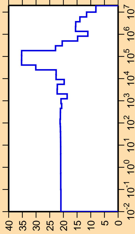
\Delta\sigma/\sigma vs. E for ^{115}\text{Cd}(n,\text{el.})
