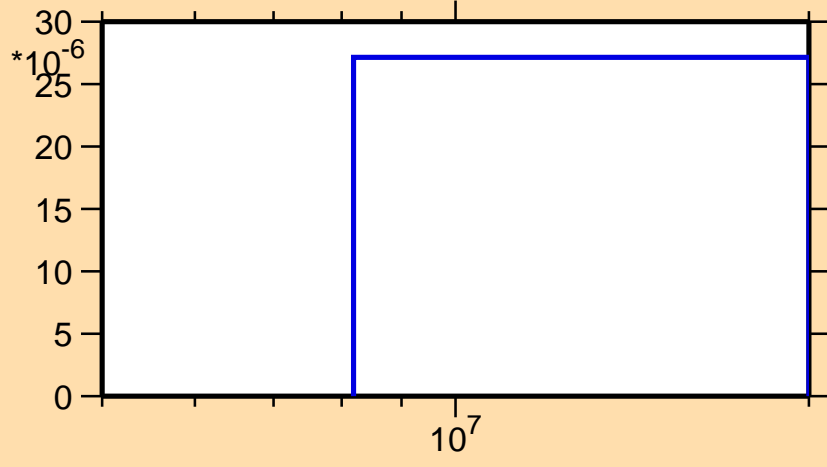
\sigma vs. E for ^{115}\text{Cd}(n,n\alpha)
