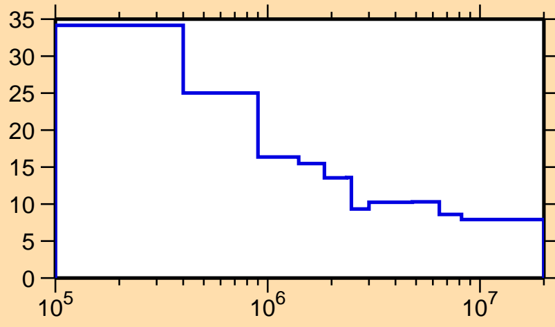
\Delta\sigma/\sigma vs. E for ^{115}\text{Cd}(n,\text{nonel.})
