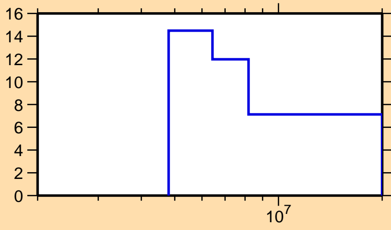
\Delta\sigma/\sigma vs. E for ^{115}\text{Cd}(n,\text{el.})
