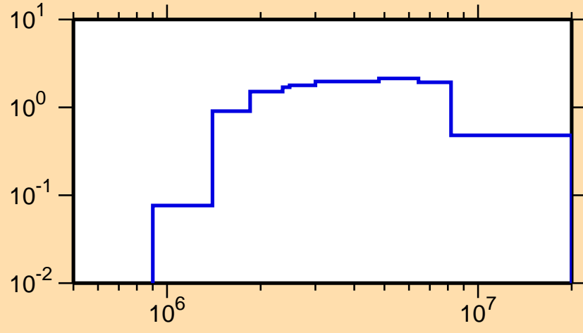
\sigma vs. E for ^{115}\text{Cd}(n,n\text{cont.})
