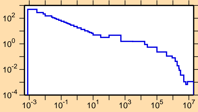
\sigma vs. E for ^{115}\text{Cd}(n,\gamma)
