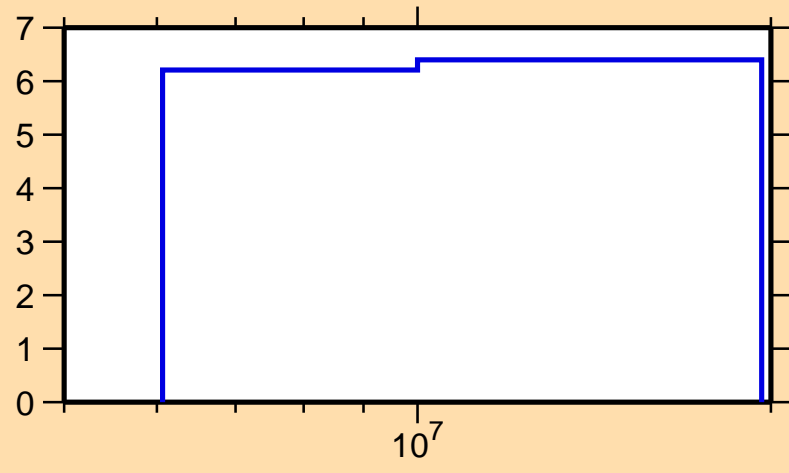
\Delta\sigma/\sigma vs. E for ^{116}\text{Cd}(n,\text{el.})
