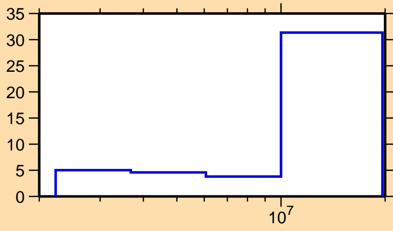
\Delta\sigma/\sigma vs. E for ^{116}\text{Cd}(n,\text{inel.})
