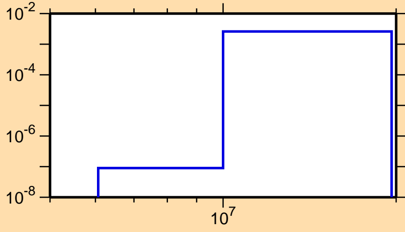
\sigma vs. E for ^{116}\text{Cd}(n,p)
