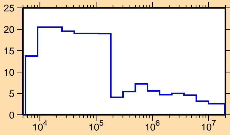
\Delta\sigma/\sigma vs. E for ^{116}\text{Cd}(n,\text{nonel.})
