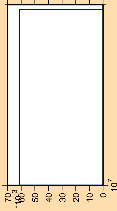
\Delta\sigma/\sigma vs. E for ^{116}\text{Cd}(n,2n\alpha)
