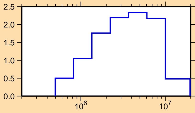
\sigma vs. E for ^{116}\text{Cd}(n,\text{inel.})
