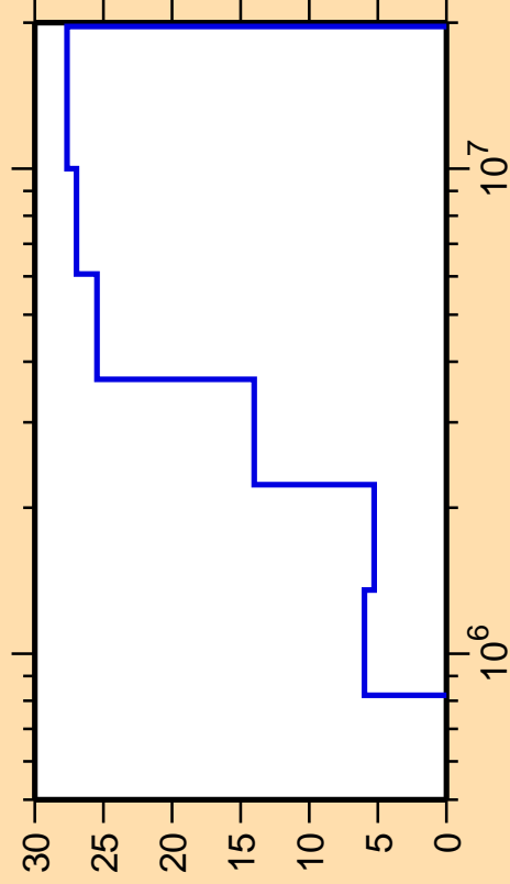
\Delta\sigma/\sigma vs. E for ^{116}\text{Cd}(n,n_2)
