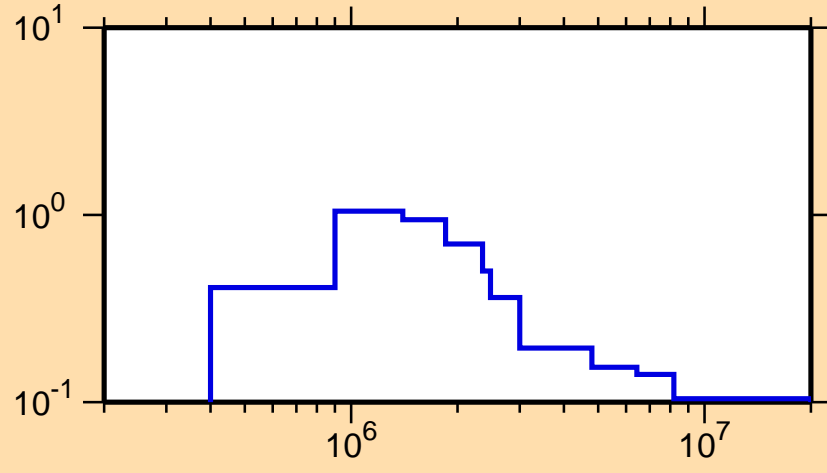
\sigma vs. E for ^{116}\text{Cd}(n,n_1)
