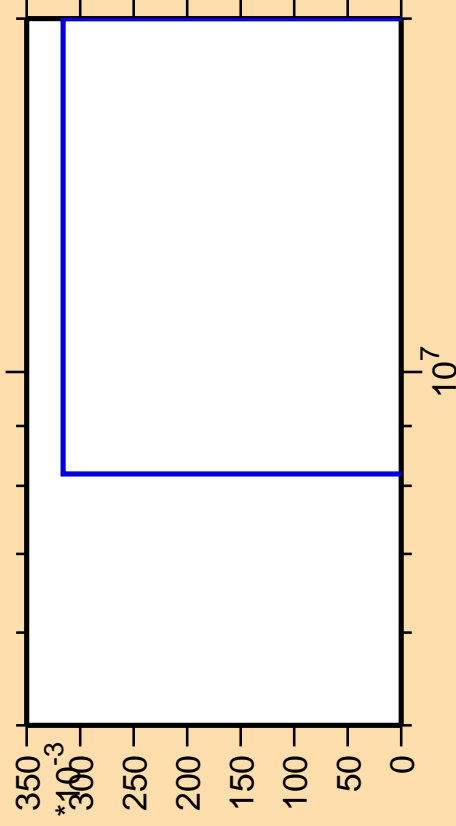
\Delta\sigma/\sigma vs. E for ^{116}\text{Cd}(n,nt)
