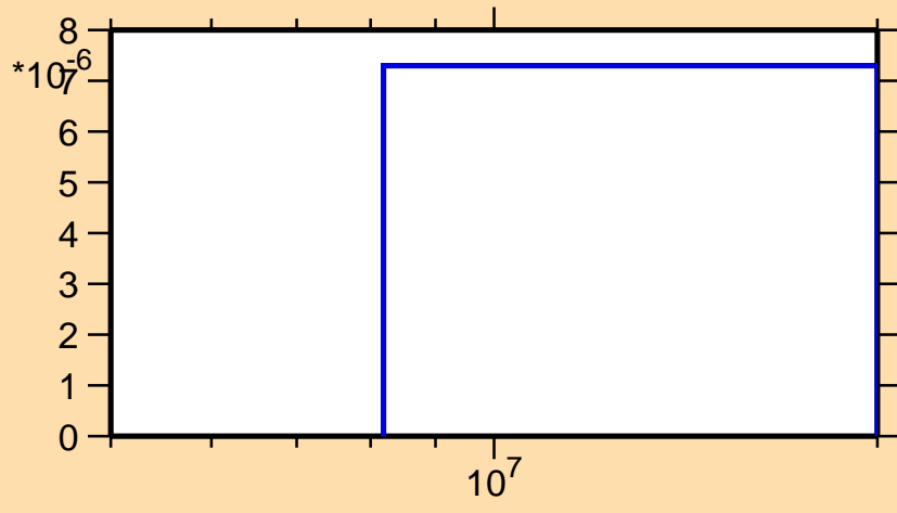
\sigma vs. E for ^{116}\text{Cd}(n,n\alpha)
