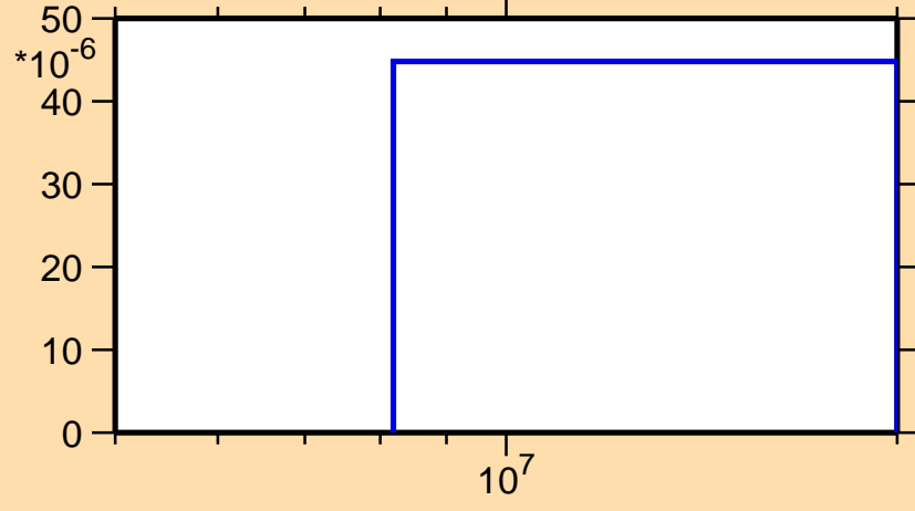
\sigma vs. E for ^{116}\text{Cd}(n,np)
