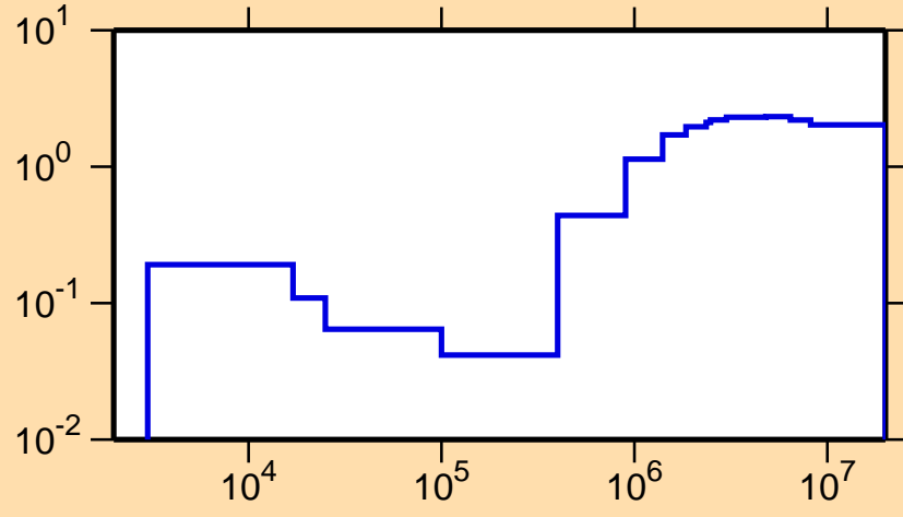
\sigma vs. E for ^{116}\text{Cd}(n,\text{nonel.})
