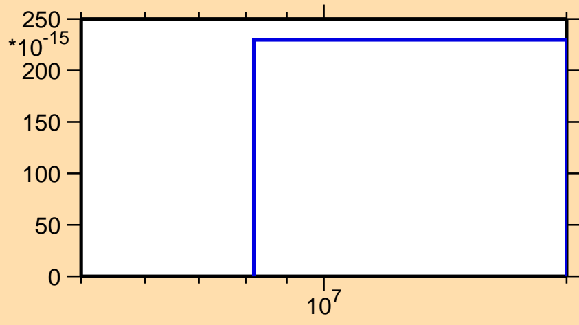
\sigma vs. E for ^{116}\text{Cd}(n,\text{nd})
