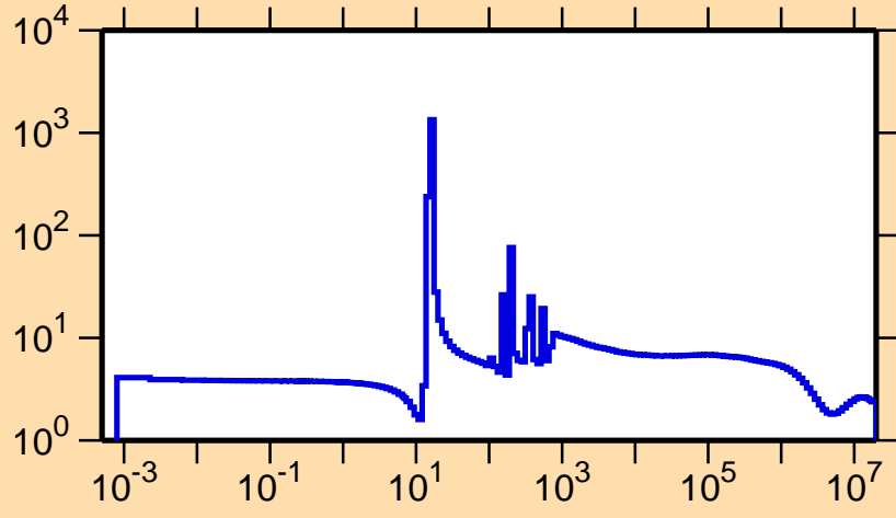
\sigma vs. E for ^{117}\text{Cd}(n,\text{el.})
