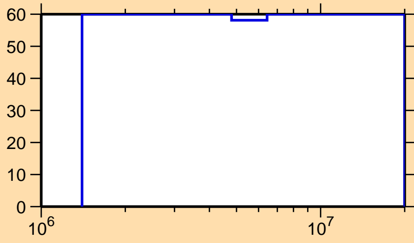
\Delta\sigma/\sigma vs. E for ^{117}\text{Cd}(n,\gamma)
