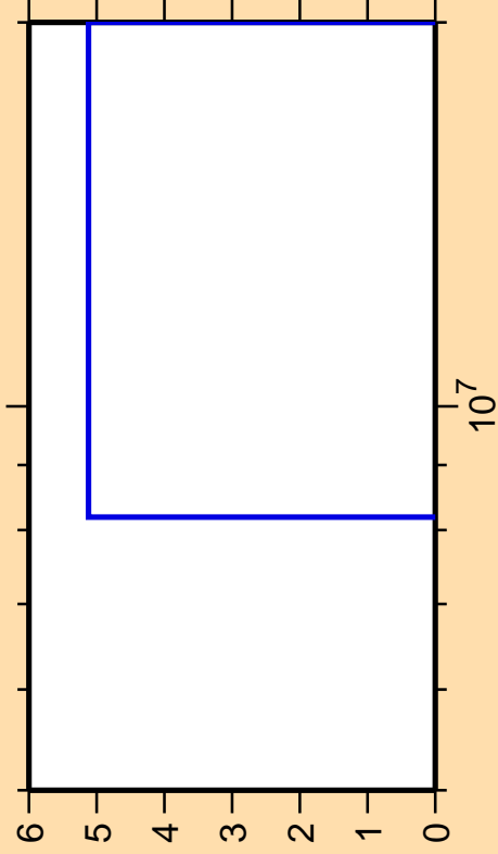
\Delta\sigma/\sigma vs. E for ^{117}\text{Cd}(n,2np)
