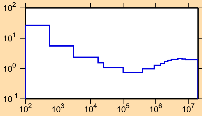
\sigma vs. E for ^{117}\text{Cd}(n,\text{nonel.})
