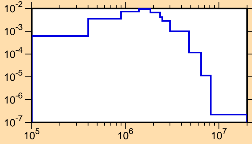
\sigma vs. E for ^{117}\text{Cd}(n,n_4)
