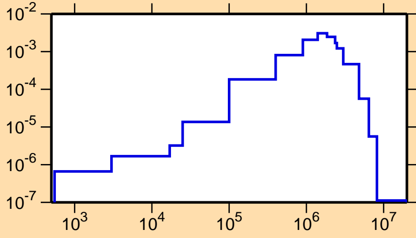
\sigma vs. E for ^{117}\text{Cd}(n,n_1)
