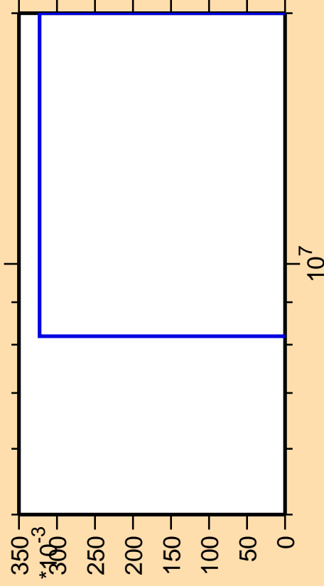
\Delta\sigma/\sigma vs. E for ^{118}\text{Cd}(n,nt)
