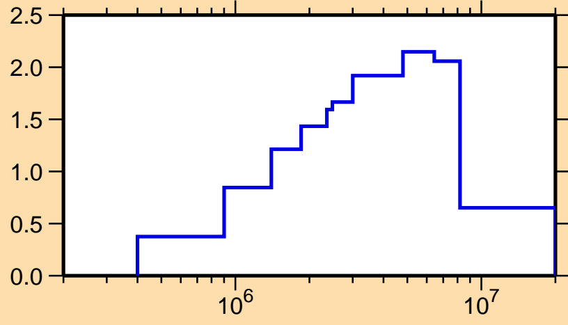
\sigma vs. E for ^{118}\text{Cd}(n,\text{inel.})
