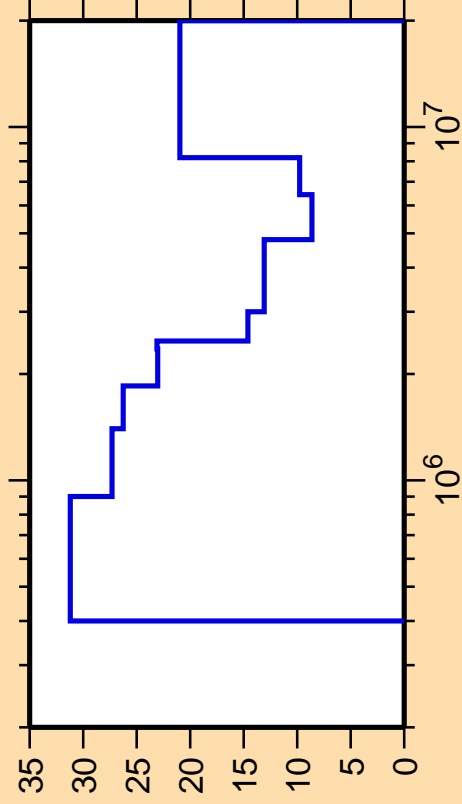
\Delta\sigma/\sigma vs. E for ^{118}\text{Cd}(n,\text{inel.})
