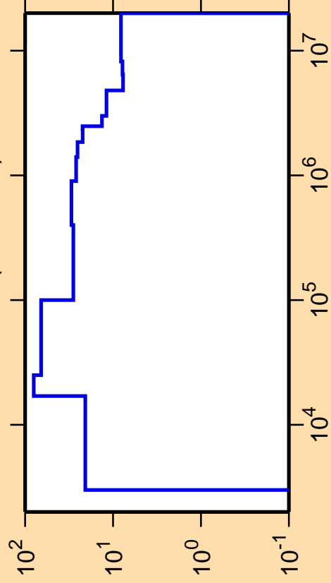
\Delta\sigma/\sigma vs. E for ^{118}\text{Cd}(n,\text{nonel.})
