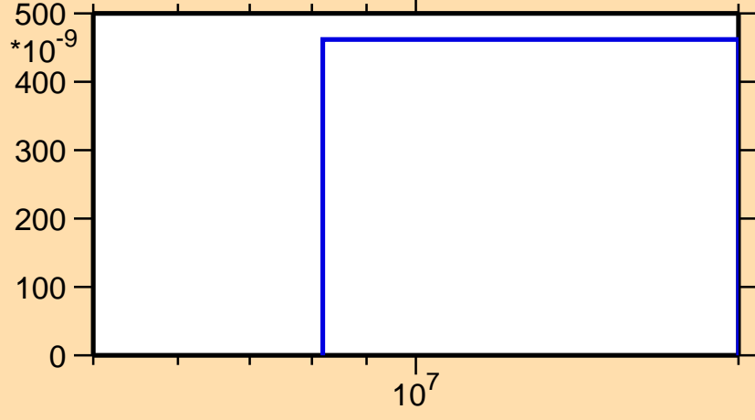
\sigma vs. E for ^{118}\text{Cd}(n,n\alpha)
