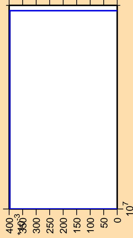
\Delta\sigma/\sigma vs. E for ^{119}\text{Cd}(n,nt)
