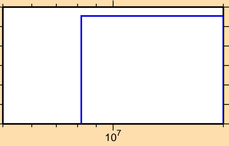
\sigma vs. E for ^{119}\text{Cd}(n,3n)
