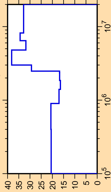
\Delta\sigma/\sigma vs. E for ^{119}\text{Cd}(n,n_3)
