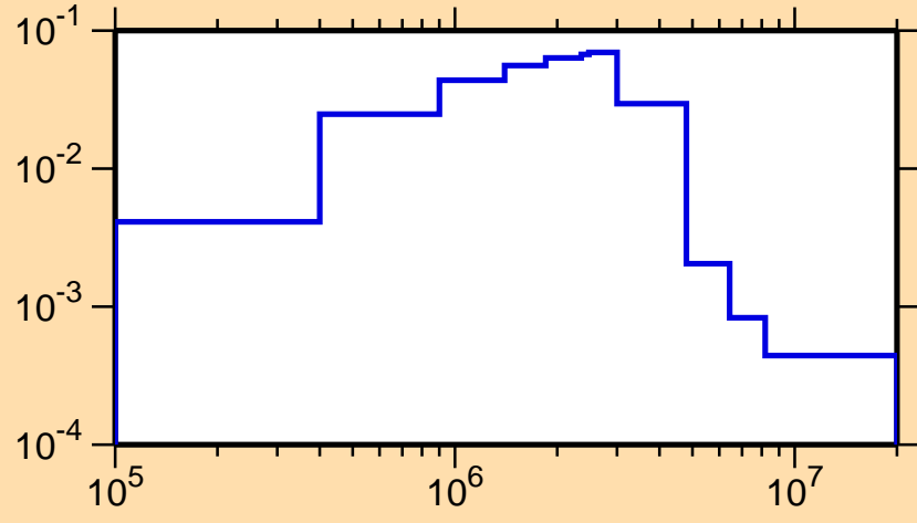
\sigma vs. E for ^{119}\text{Cd}(n,n_3)
