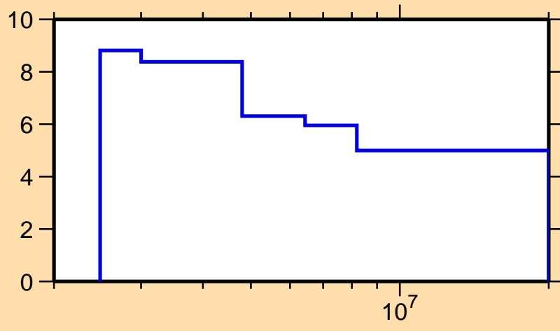
\Delta\sigma/\sigma vs. E for ^{119}\text{Cd}(n,n\text{onel.})
