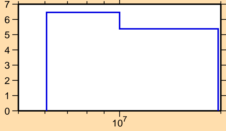
\Delta\sigma/\sigma vs. E for ^{119}\text{Cd}(n,2n)
