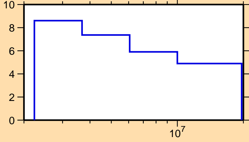
\Delta\sigma/\sigma vs. E for ^{119}\text{Cd}(n,n\text{onel.})
