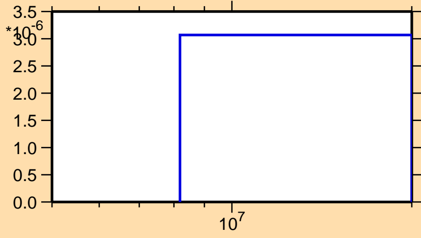
\sigma vs. E for ^{119}\text{Cd}(n,t)
