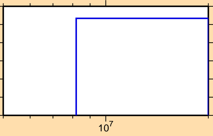
\sigma vs. E for ^{119}\text{Cd}(n,np)
