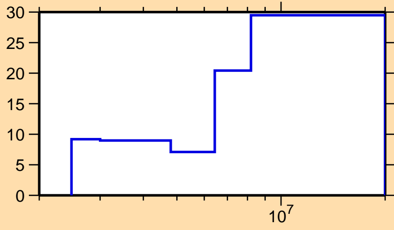
\Delta\sigma/\sigma vs. E for ^{119}\text{Cd}(n,n\text{cont.})
