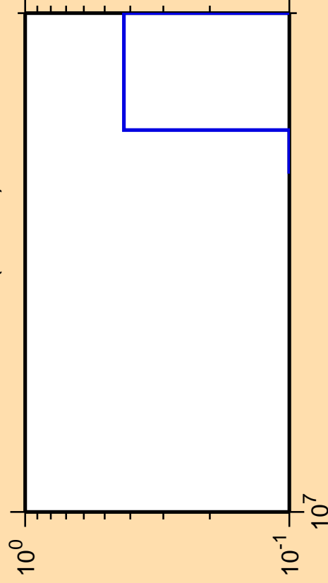
\Delta\sigma/\sigma vs. E for ^{120}\text{Cd}(n,2n\alpha)
