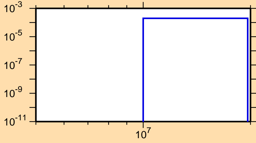
\sigma vs. E for ^{120}\text{Cd}(n,p)
