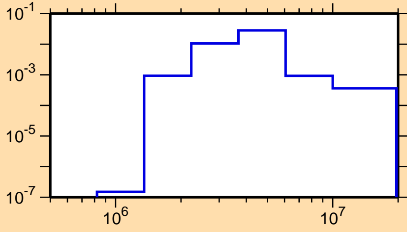
\sigma vs. E for ^{120}\text{Cd}(n,n_4)
