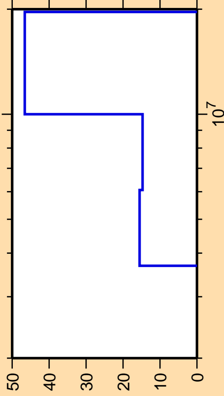
\Delta\sigma/\sigma vs. E for ^{120}\text{Cd}(n,n\text{cont.})
