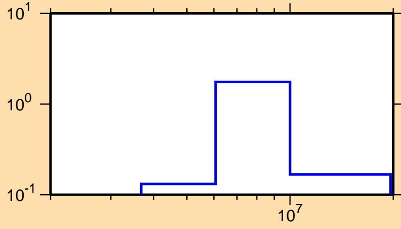
\sigma vs. E for ^{120}\text{Cd}(n,n\text{cont.})
