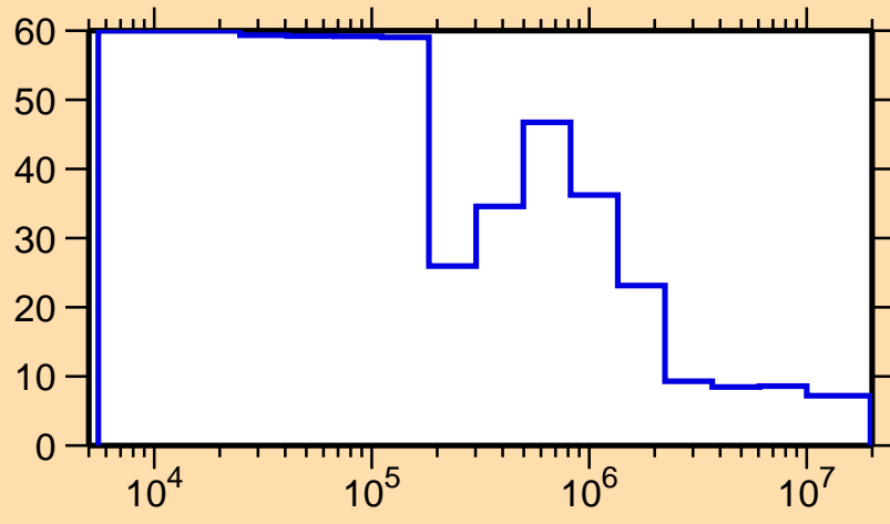
\Delta\sigma/\sigma vs. E for ^{120}\text{Cd}(n,\text{nonel.})
