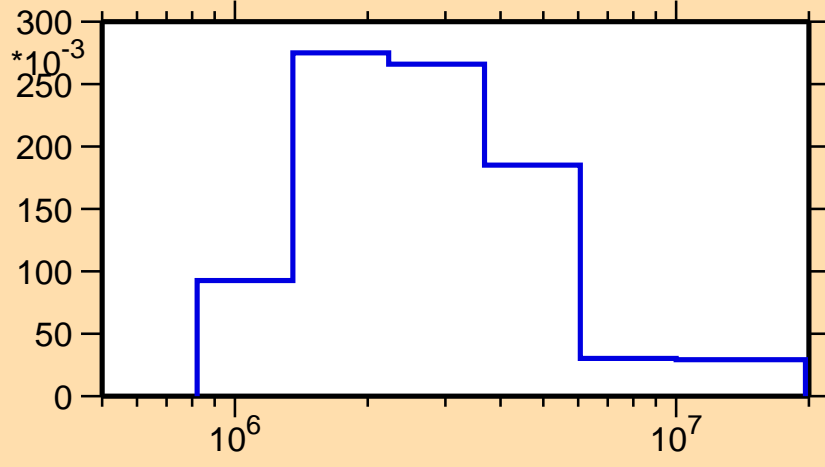
\sigma vs. E for ^{120}\text{Cd}(n,n_2)
