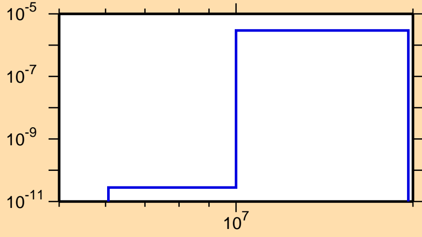
\sigma vs. E for ^{120}\text{Cd}(n,\alpha)
