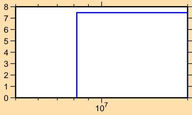
\Delta\sigma/\sigma vs. E for ^{120}\text{Cd}(n,\text{nonel.})
