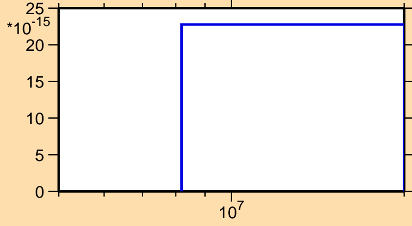
\sigma vs. E for ^{120}\text{Cd}(n,nt)
