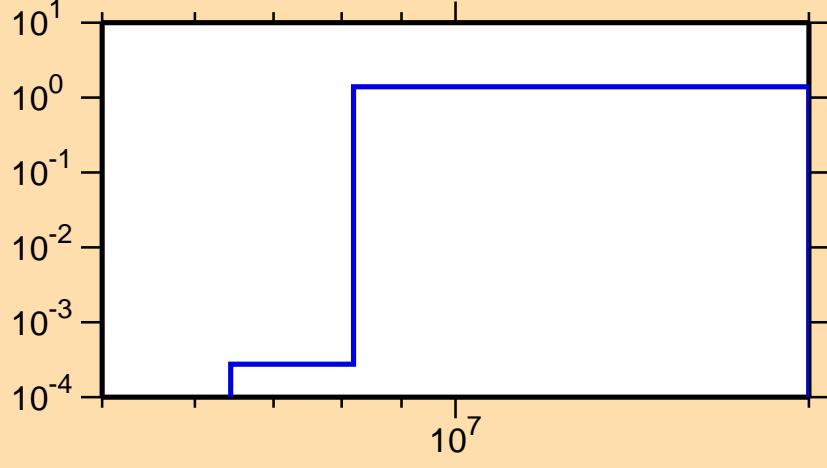
\sigma vs. E for ^{120}\text{Cd}(n,2n)
