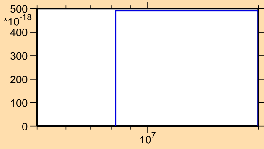
\sigma vs. E for ^{120}\text{Cd}(n,\text{nd})
