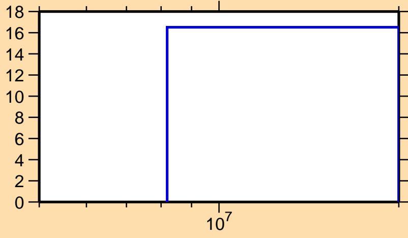
\Delta\sigma/\sigma vs. E for ^{120}\text{Cd}(n,n\text{cont.})
