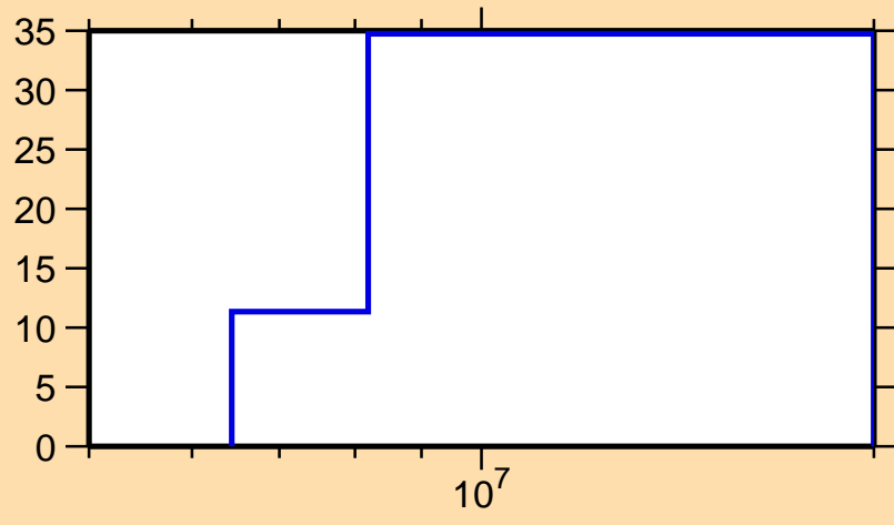
\Delta\sigma/\sigma vs. E for ^{120}\text{Cd}(n,\text{inel.})
