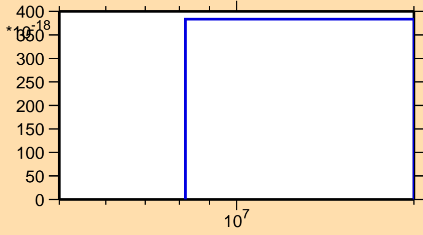
\sigma vs. E for ^{120}\text{Cd}(n,2n\alpha)
