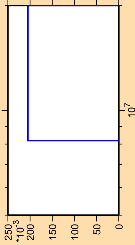
\Delta\sigma/\sigma vs. E for ^{120}\text{Cd}(n,nt)
