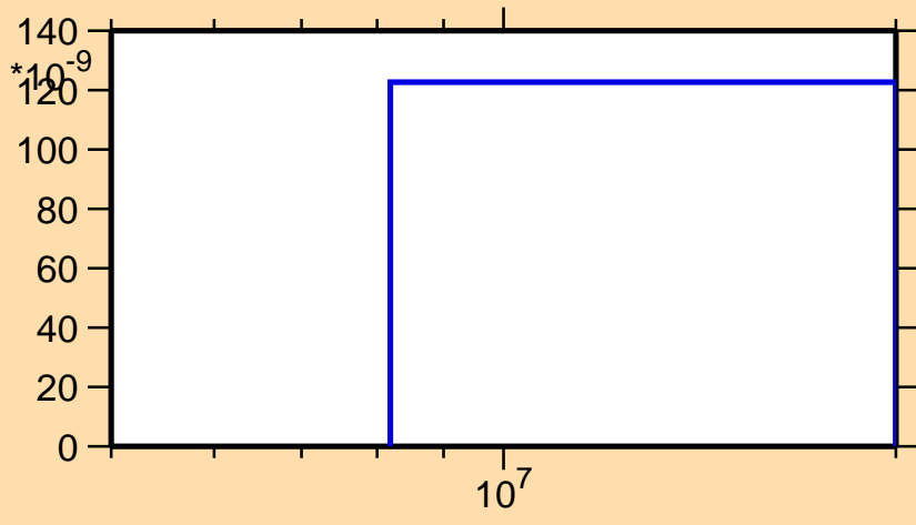
\sigma vs. E for ^{120}\text{Cd}(n,t)
