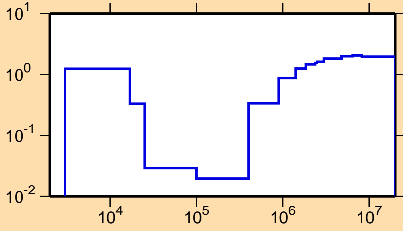
\sigma vs. E for ^{120}\text{Cd}(n,\text{nonel.})
