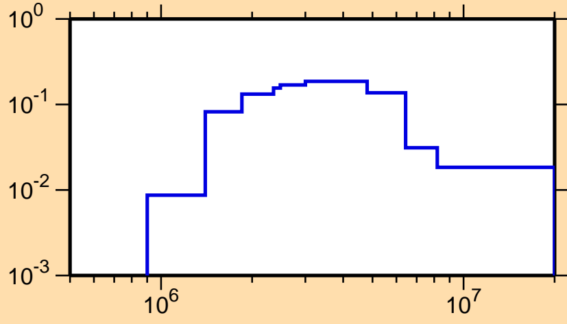
\sigma vs. E for ^{120}\text{Cd}(n,n_3)
