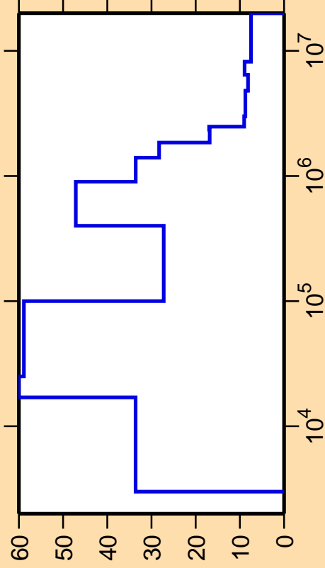
\Delta\sigma/\sigma vs. E for ^{120}\text{Cd}(n,\text{nonel.})
