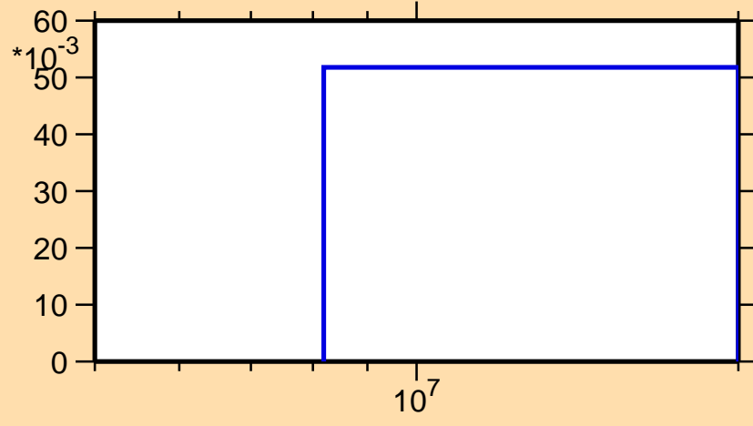
\sigma vs. E for ^{120}\text{Cd}(n,3n)
