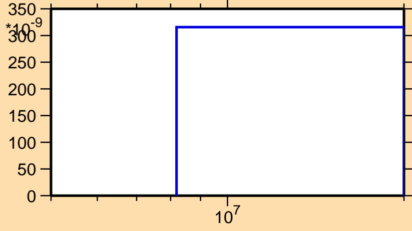
\sigma vs. E for ^{120}\text{Cd}(n,np)
