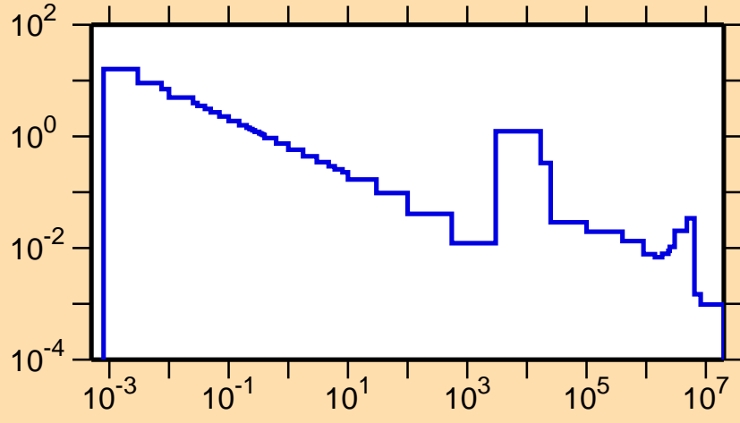
\sigma vs. E for ^{120}\text{Cd}(n,\gamma)
