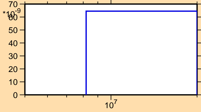
\sigma vs. E for ^{120}\text{Cd}(n,n\alpha)
