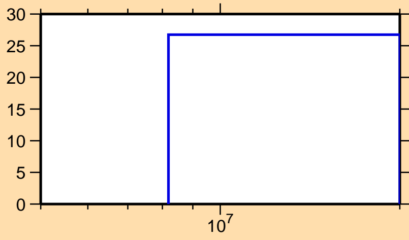
\Delta\sigma/\sigma vs. E for ^{120}\text{Cd}(n,\text{el.})
