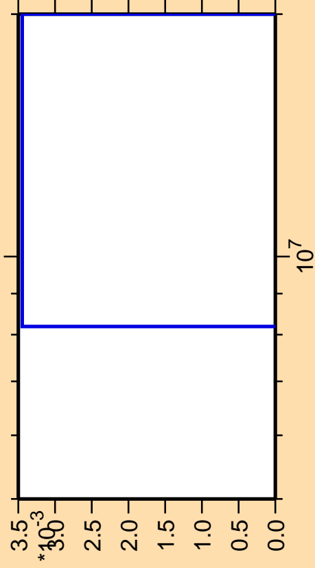
\Delta\sigma/\sigma vs. E for ^{120}\text{Cd}(n,2n\alpha)
