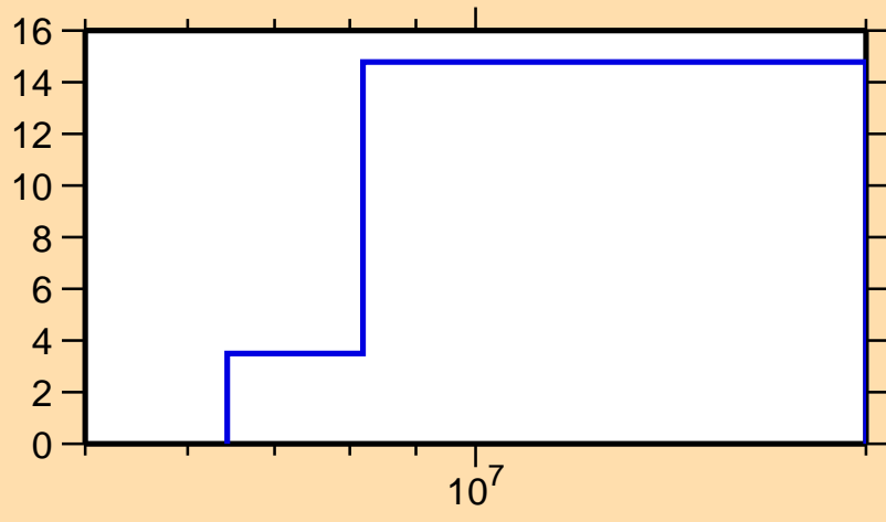
\Delta\sigma/\sigma vs. E for ^{120}\text{Cd}(n,\text{tot.})
