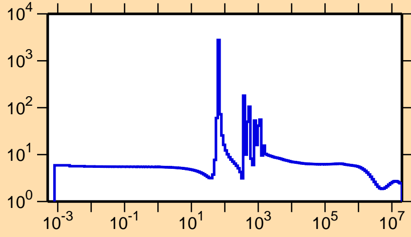
\sigma vs. E for ^{121}\text{Cd}(n,\text{el.})
