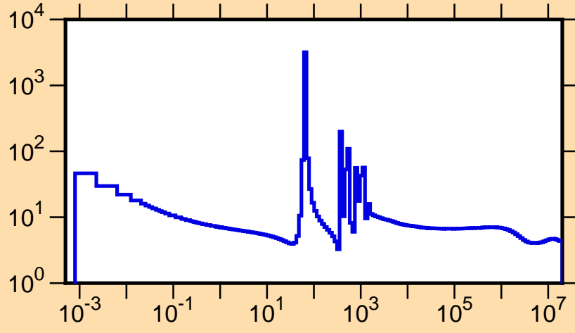
\sigma vs. E for ^{121}\text{Cd}(n,\text{tot.})
