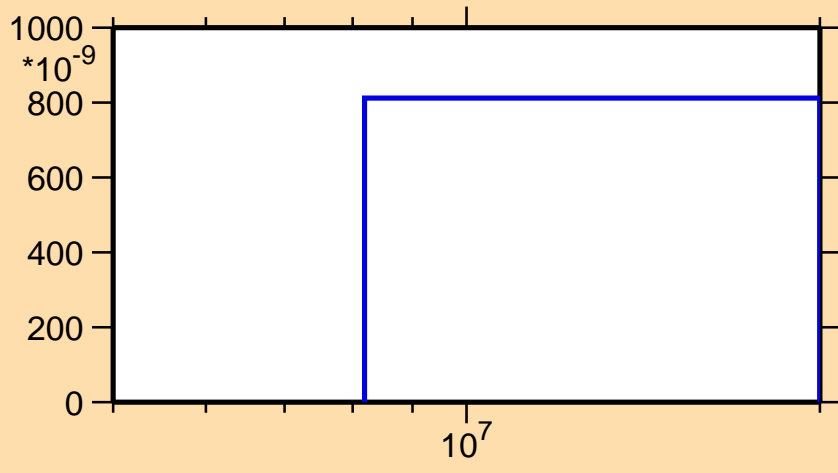
\sigma vs. E for ^{121}\text{Cd}(n,np)
