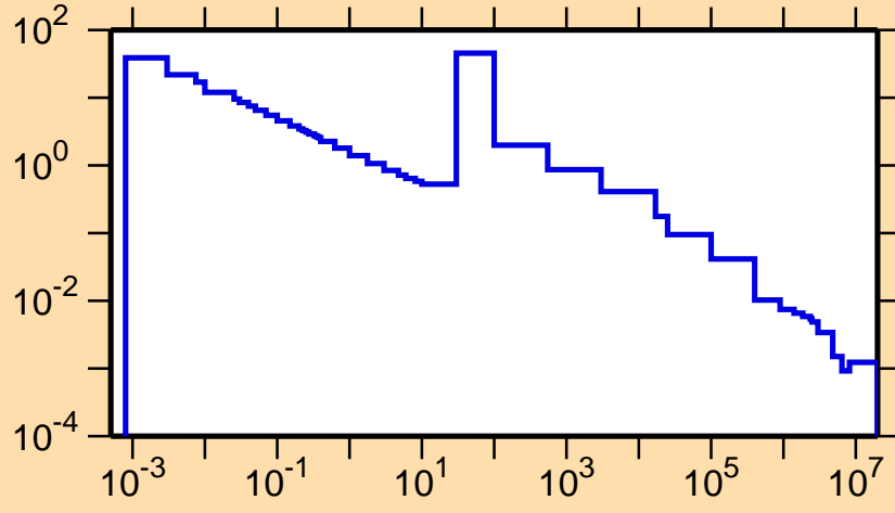
\sigma vs. E for ^{121}\text{Cd}(n,\gamma)
