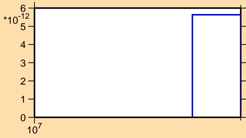
\sigma vs. E for ^{121}\text{Cd}(n,2np)
