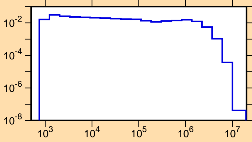
\sigma vs. E for ^{121}\text{Cd}(n,n_1)
