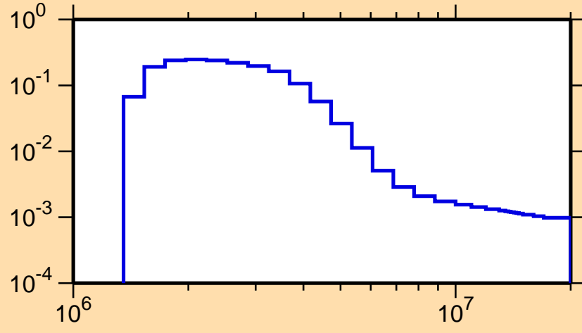
\sigma vs. E for ^{122}\text{Cd}(n,n_4)
