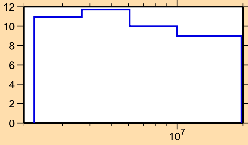
\Delta\sigma/\sigma vs. E for ^{122}\text{Cd}(n,n\text{onel.})
