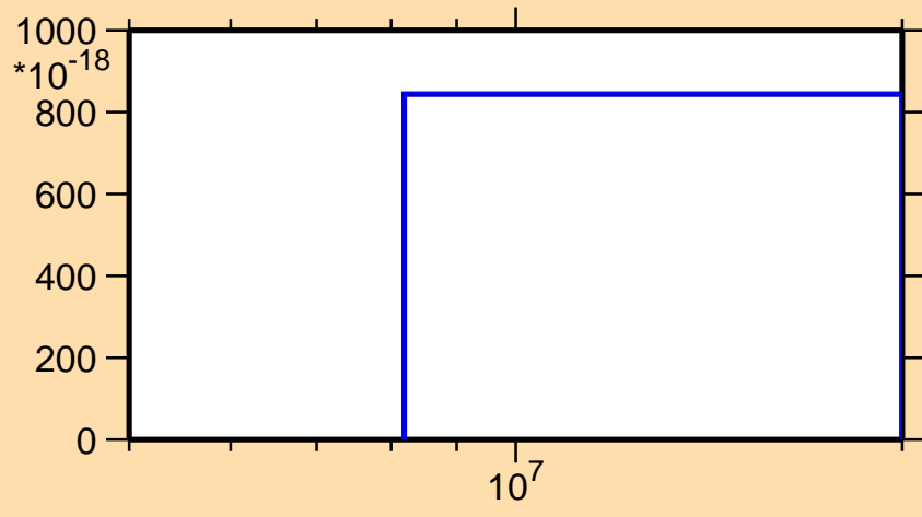
\sigma vs. E for ^{122}\text{Cd}(n,nt)
