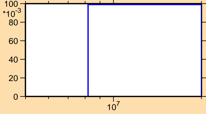
\sigma vs. E for ^{122}\text{Cd}(n,3n)
