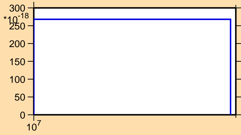
\sigma vs. E for ^{123}\text{Cd}(n,2np)
