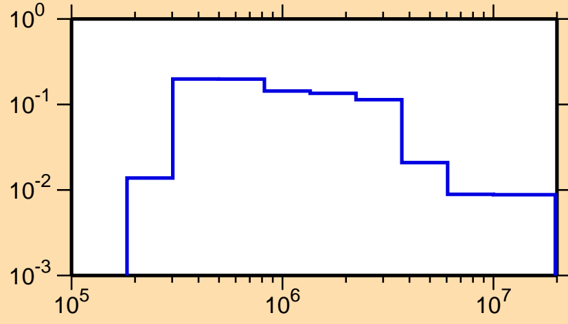
\sigma vs. E for ^{123}\text{Cd}(n,n_2)
