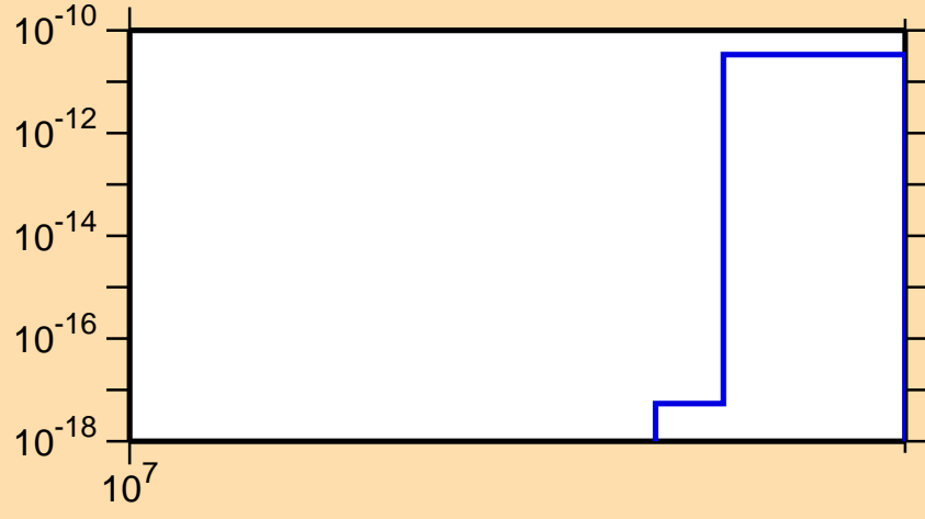
\sigma vs. E for ^{123}\text{Cd}(n,nt)
