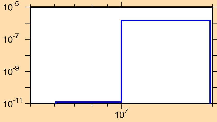
\sigma vs. E for ^{123}\text{Cd}(n,\alpha)
