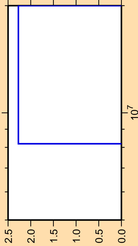
\Delta\sigma/\sigma vs. E for ^{123}\text{Cd}(n,nt)
