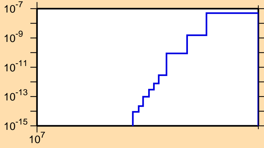
\sigma vs. E for ^{124}\text{Cd}(n,n\alpha)
