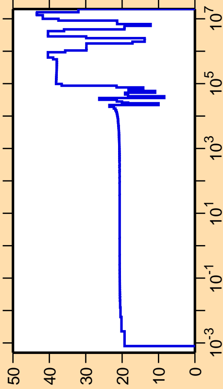
\Delta\sigma/\sigma vs. E for ^{124}\text{Cd}(n,\text{el.})
