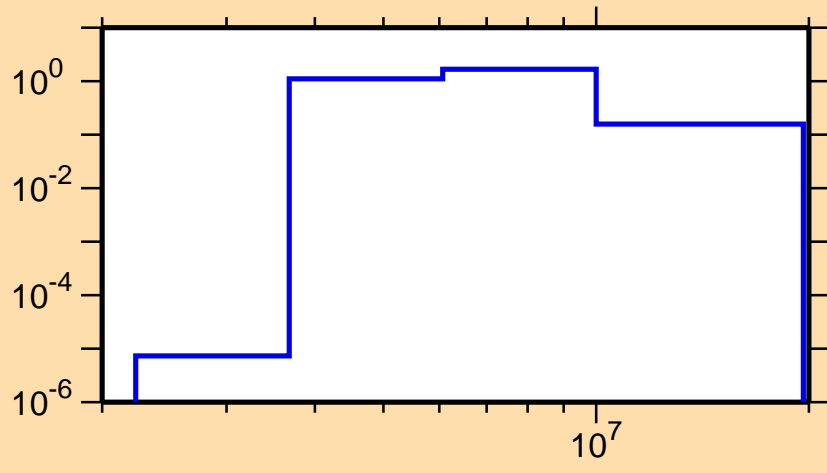
\sigma vs. E for ^{124}\text{Cd}(n,n\text{cont.})
