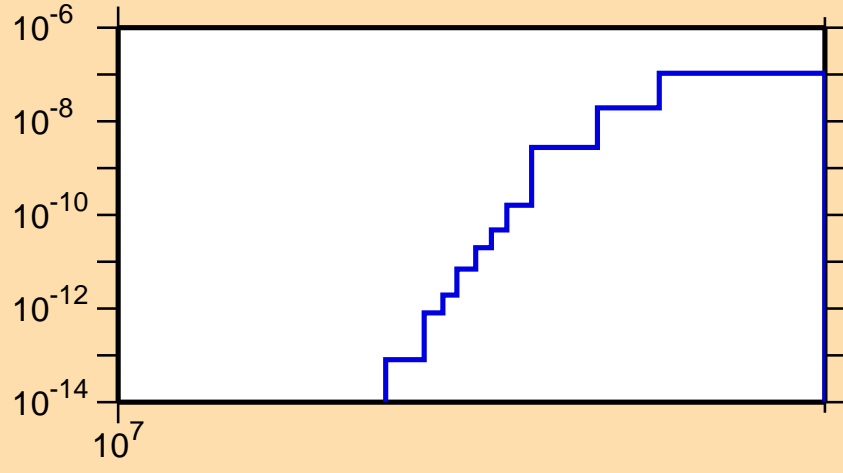
\sigma vs. E for ^{121}\text{Ce}(n,2n\alpha)
