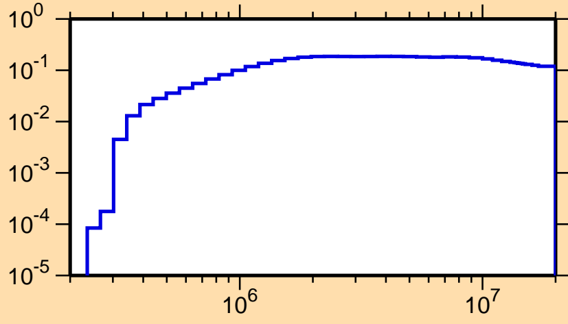
\sigma vs. E for ^{121}\text{Ce}(n,\text{inel.})
