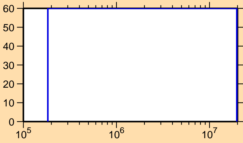
\Delta\sigma/\sigma vs. E for ^{121}\text{Ce}(n,n_1)
